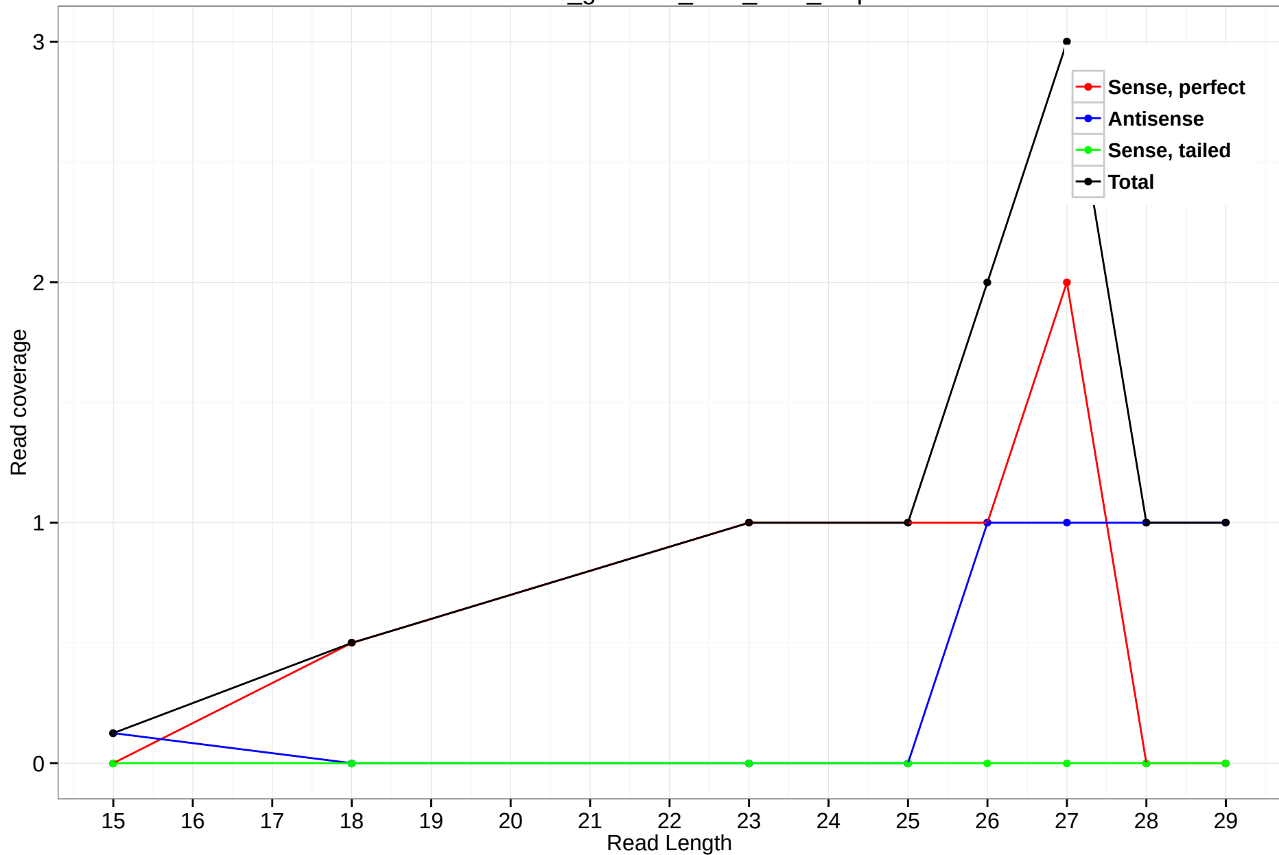
rheMac3_genscan_chr3_61.5_1.5p
