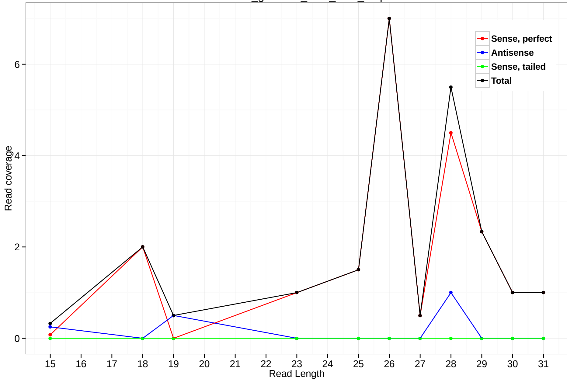
rheMac3_genscan_chr3_59.2_4.5p
