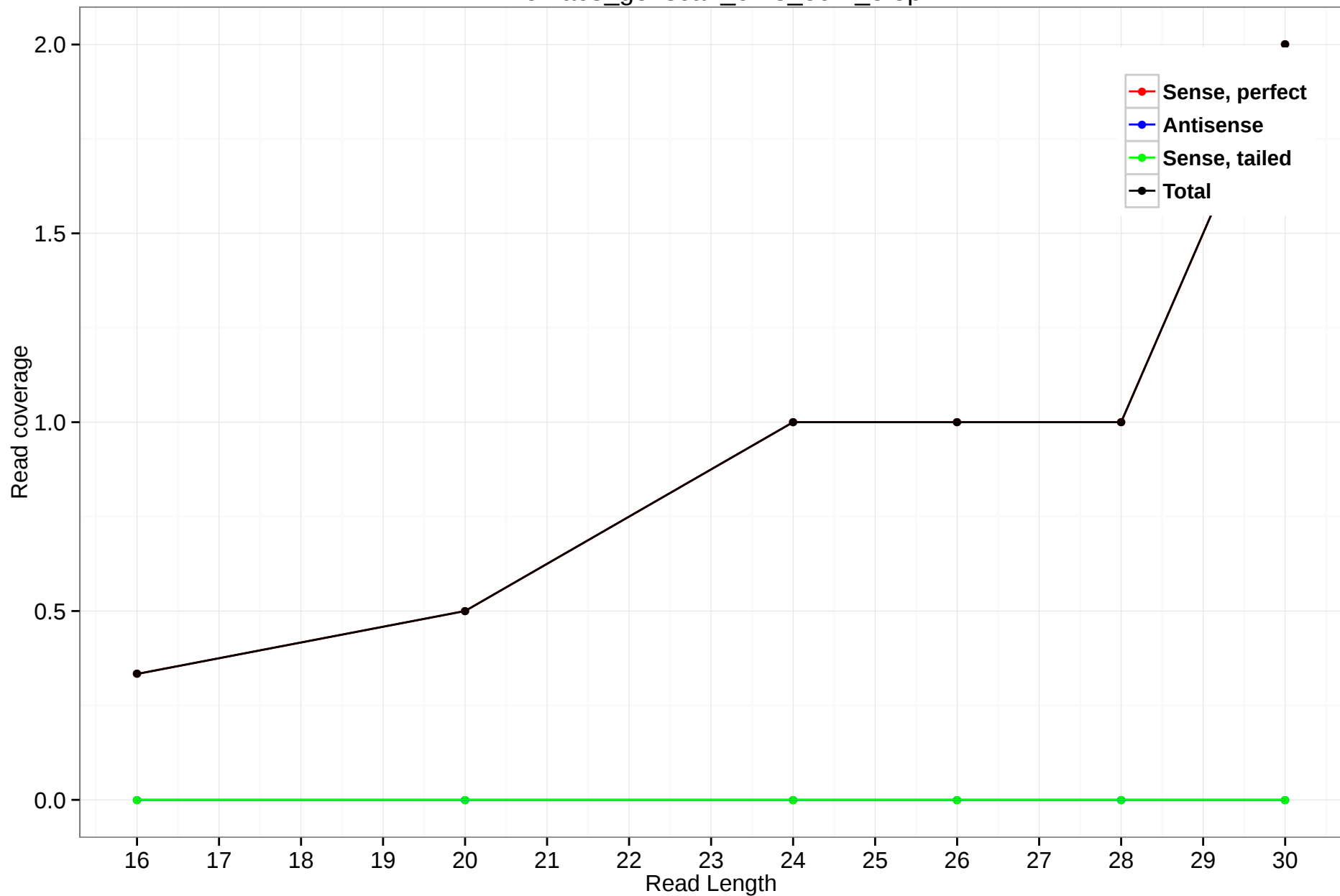
rheMac3_genscan_chr3_59.2_3.5p
