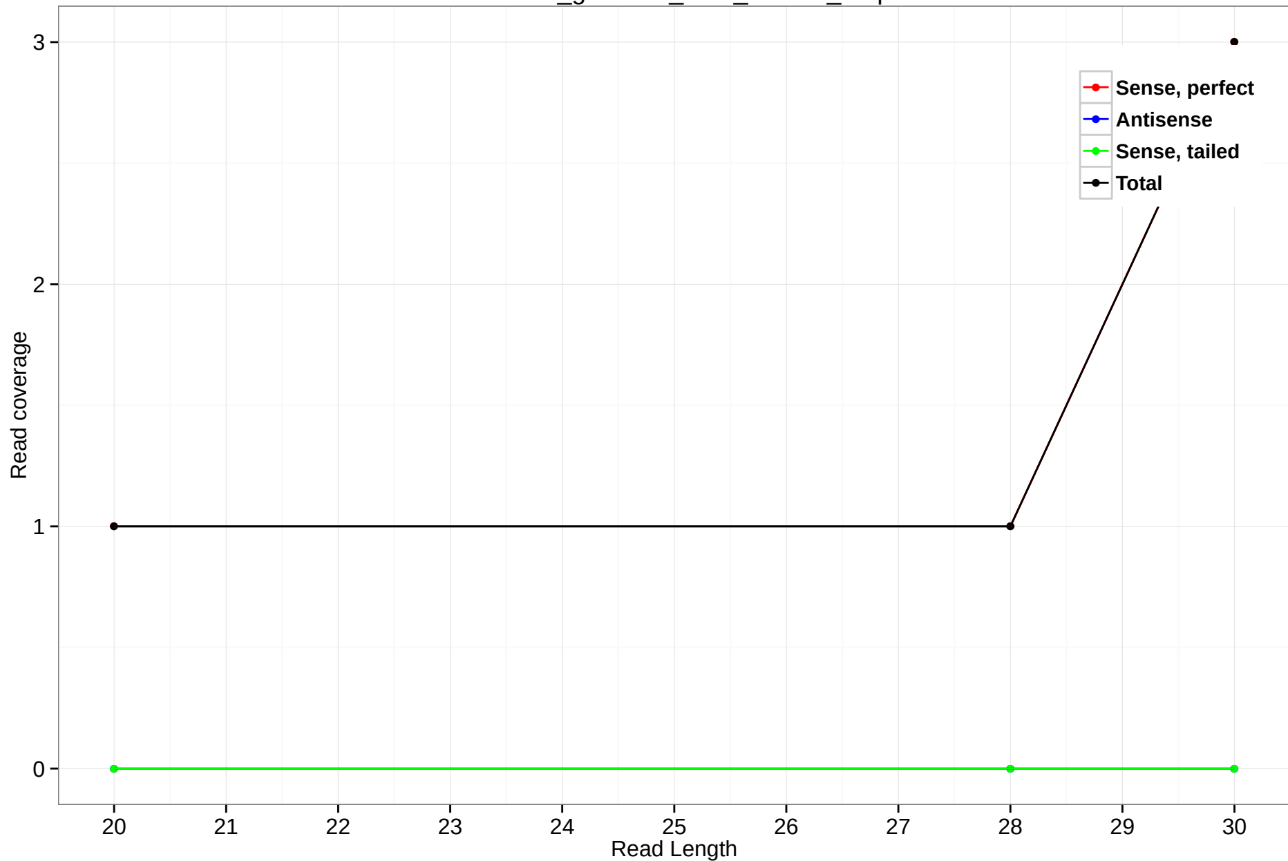
rheMac3_genscan_chr3_314.22_1.5p
