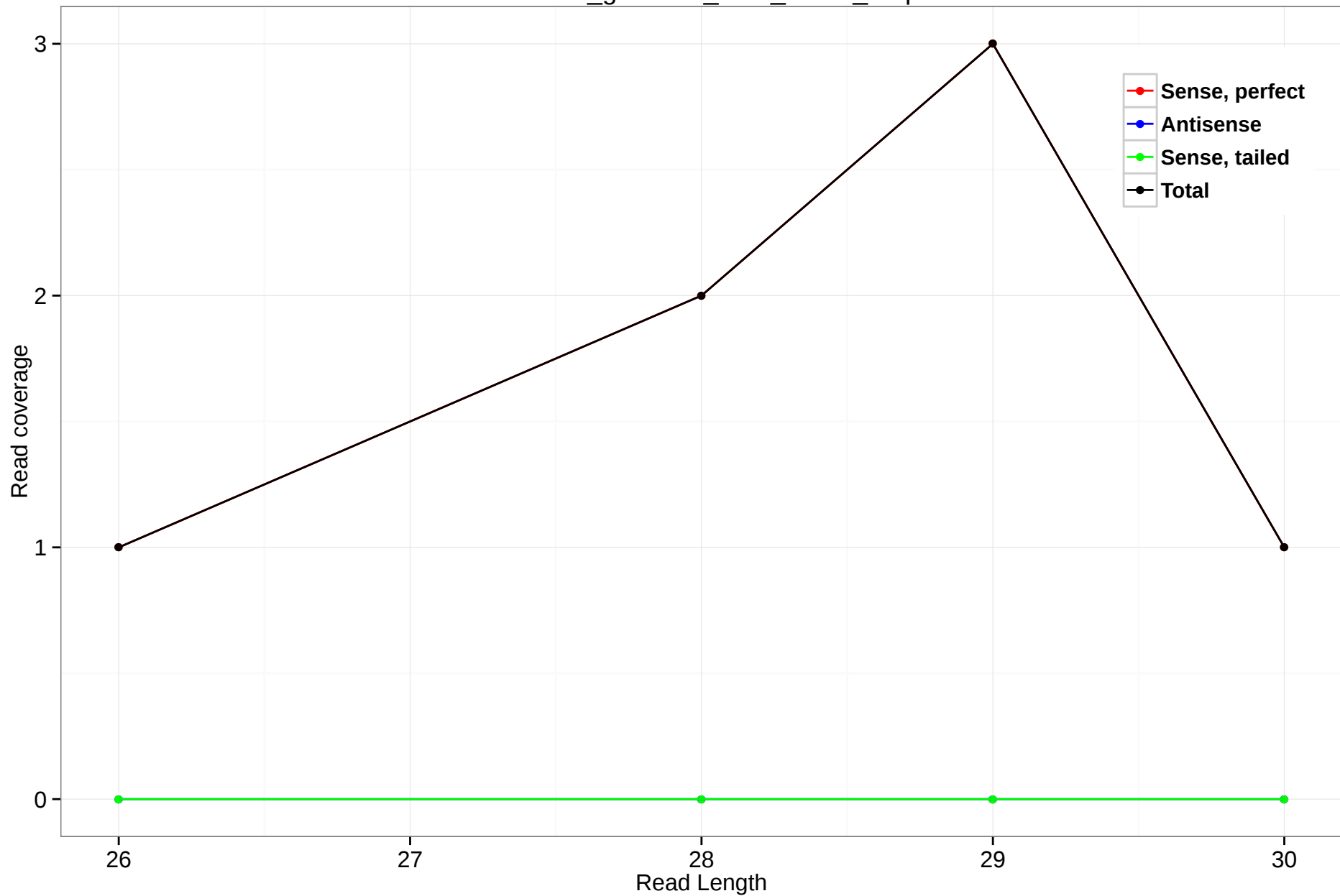
rheMac3_genscan_chr3_302.8_0.5p
