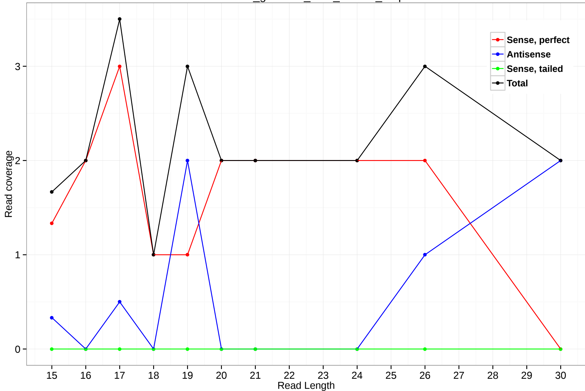
rheMac3_genscan_chr3_283.25_3.5p
