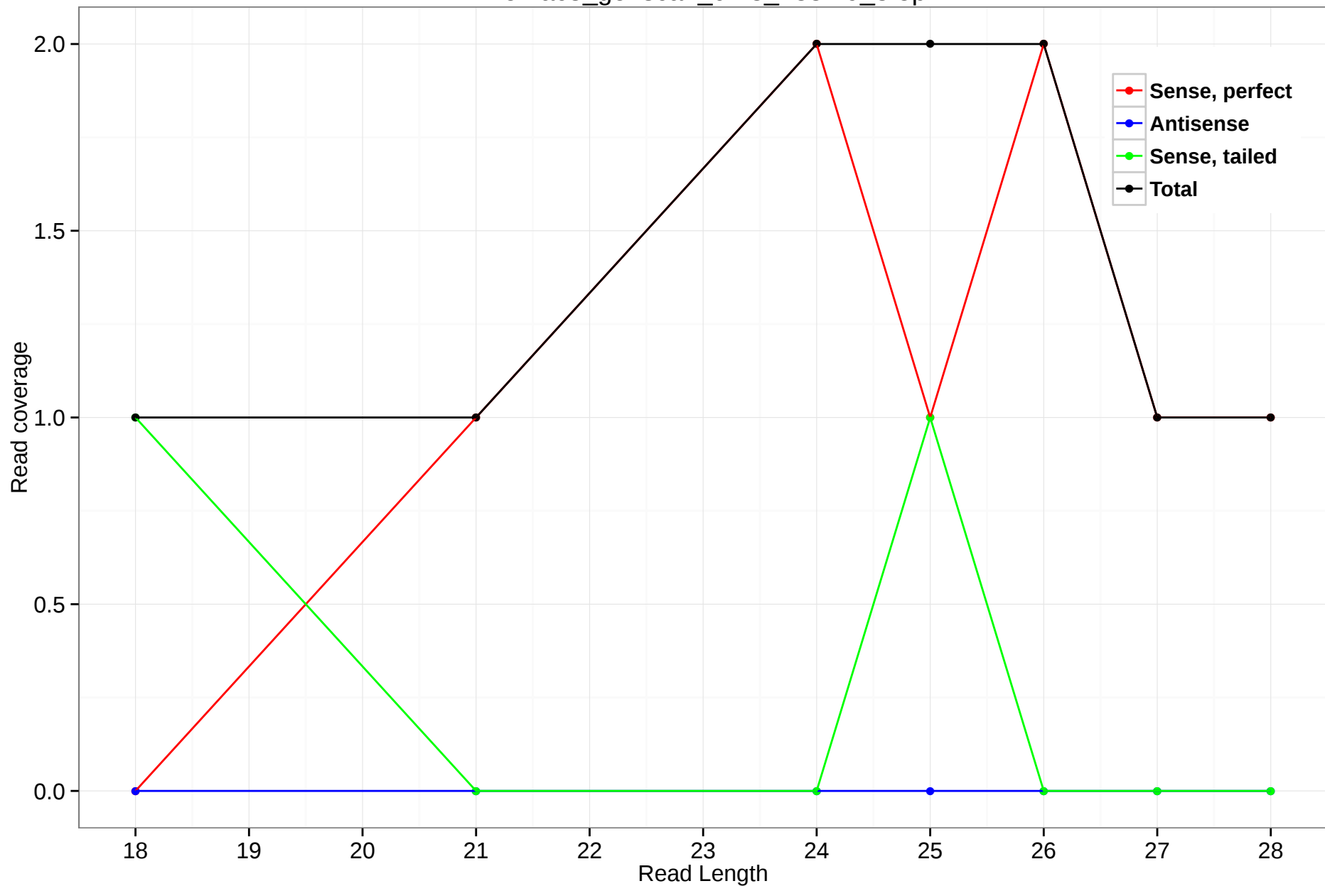
rheMac3_genscan_chr3_283.19_3.5p
