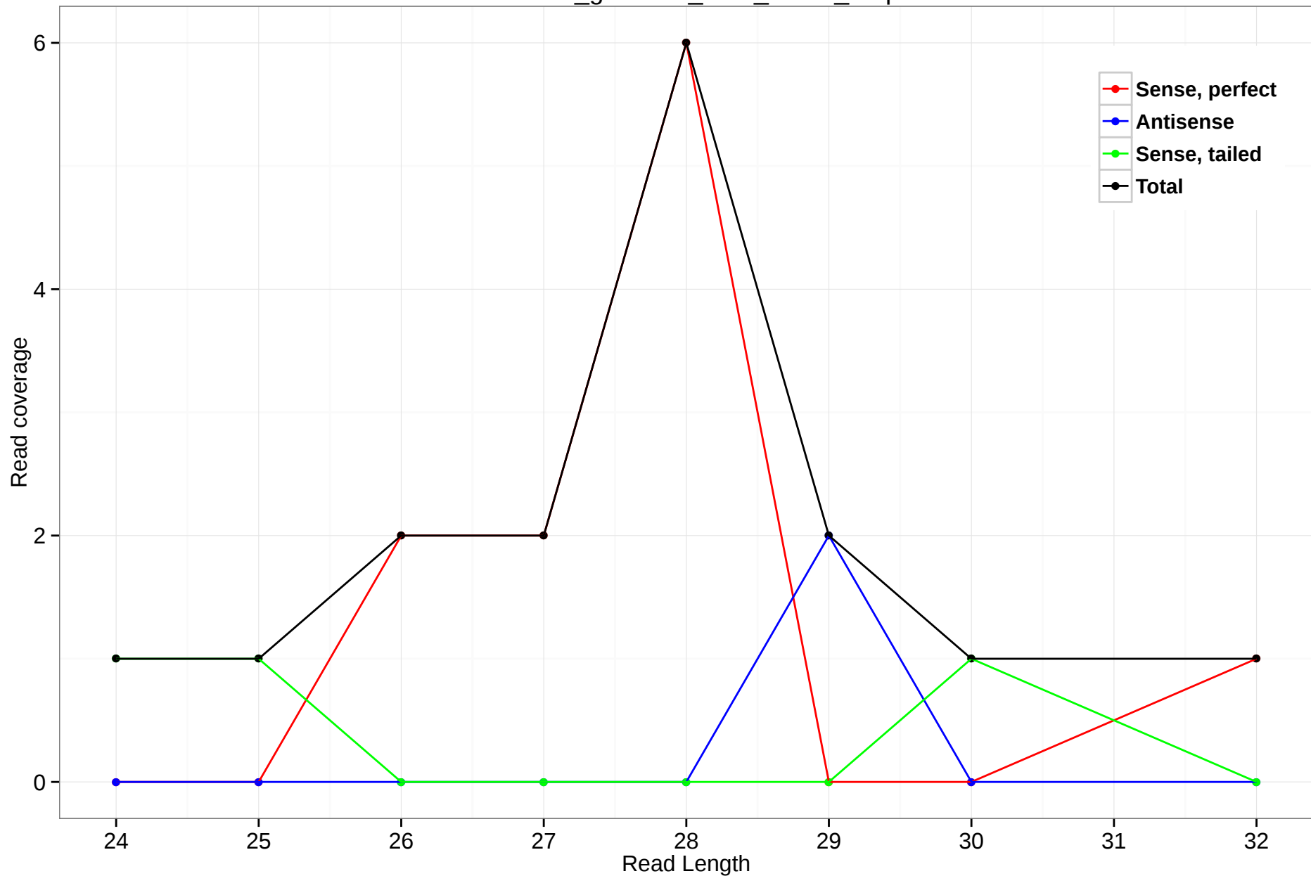
rheMac3_genscan_chr3_278.4_3.5p
