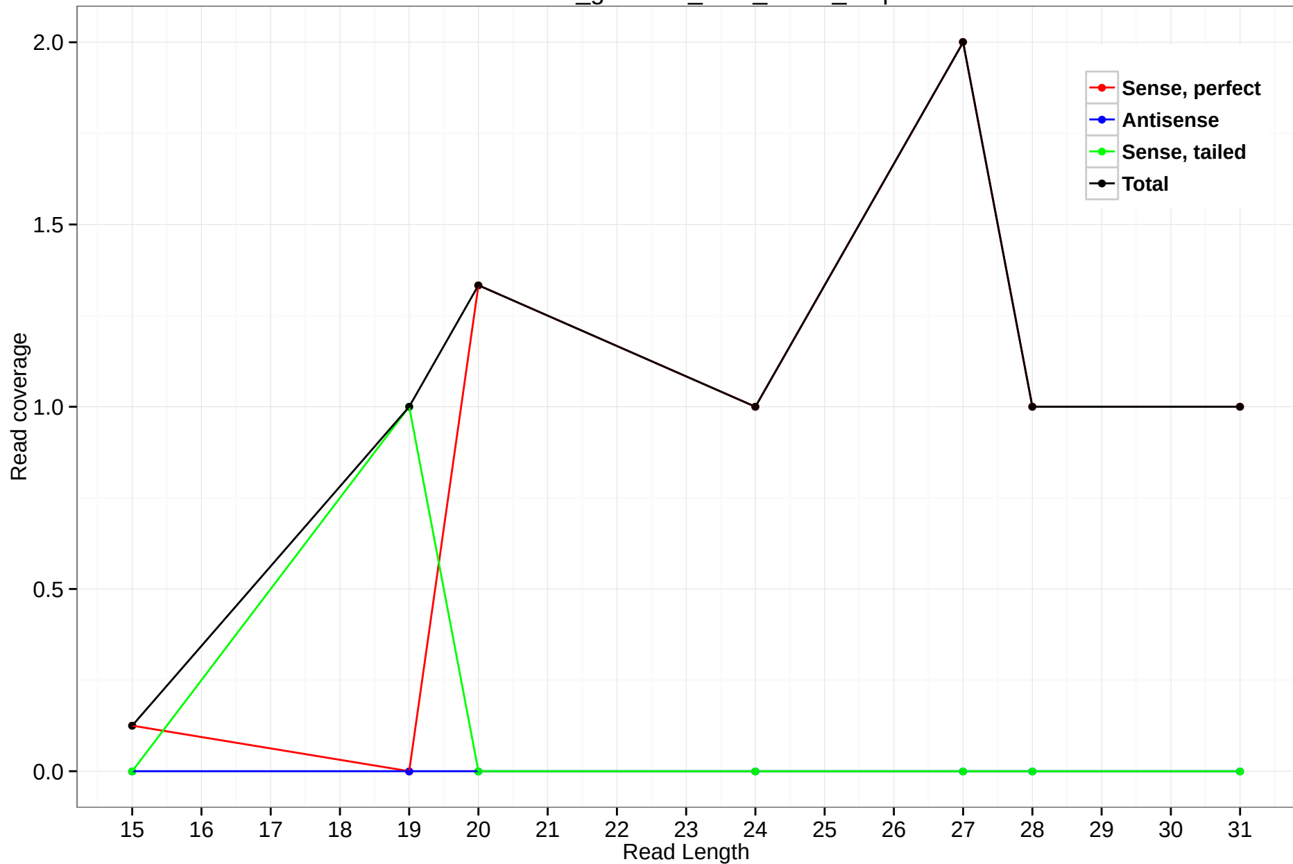
rheMac3_genscan_chr3_270.9_4.5p
