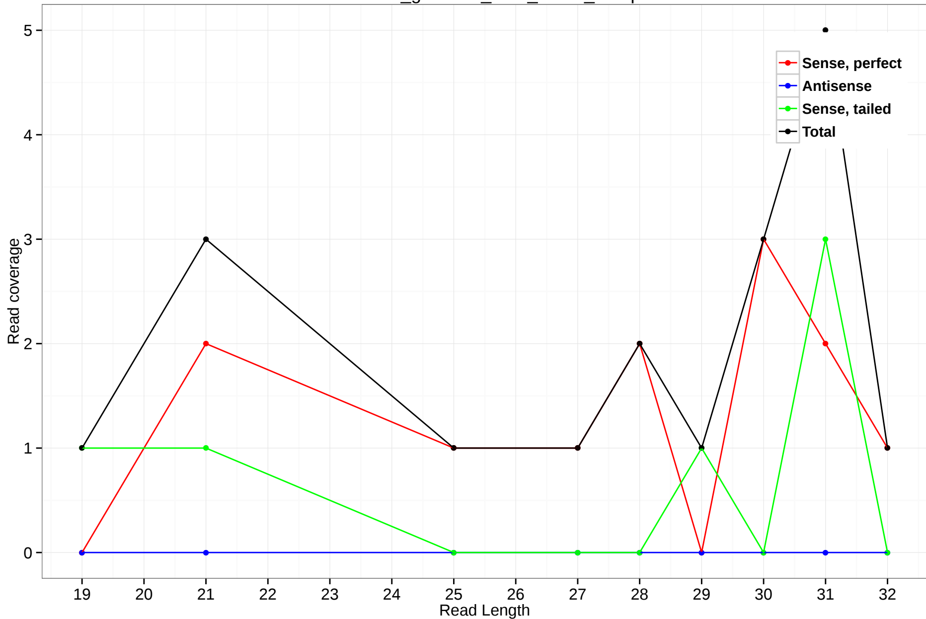
rheMac3_genscan_chr3_270.5_14.5p
