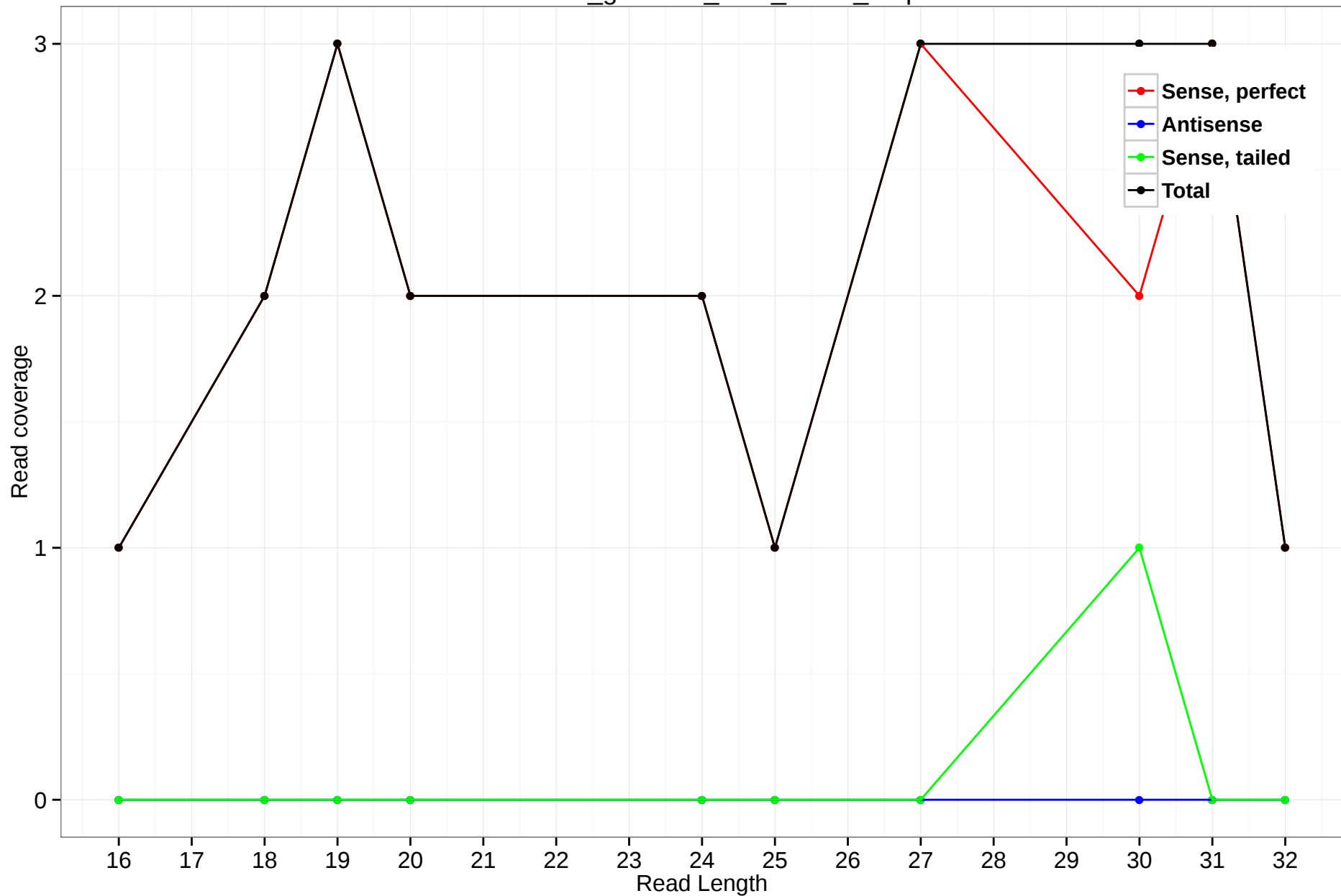
rheMac3_genscan_chr3_269.4_3.5p
