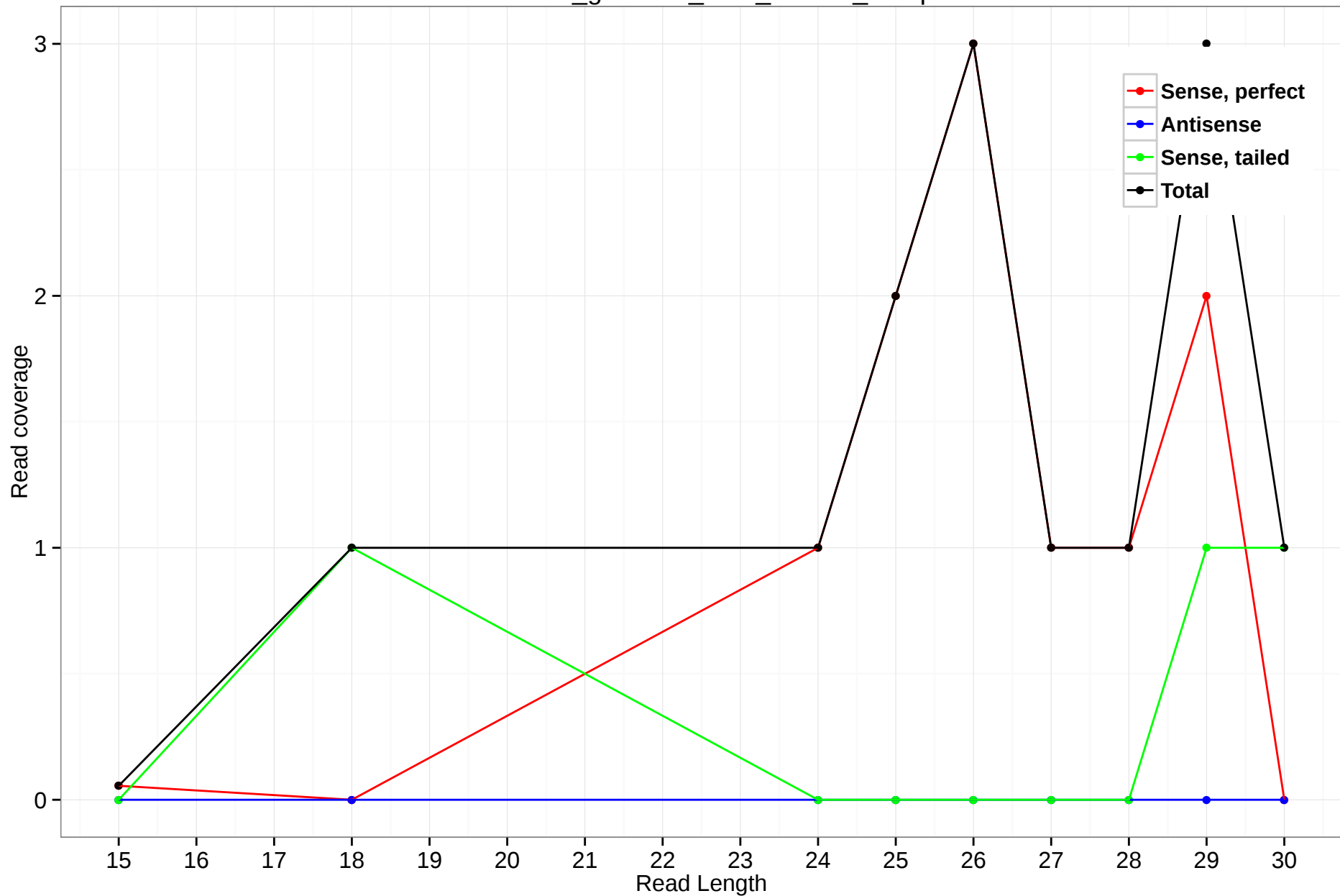
rheMac3_genscan_chr3_268.10_24.3p
