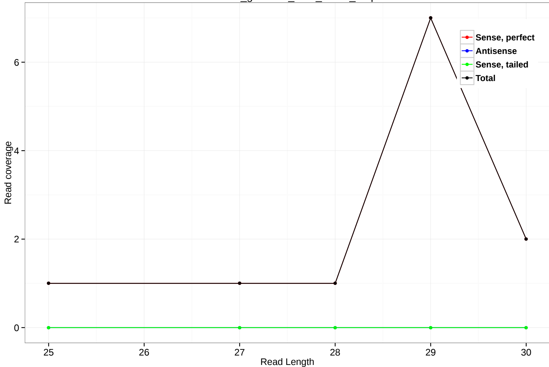
rheMac3_genscan_chr3_263.6_1.3p
