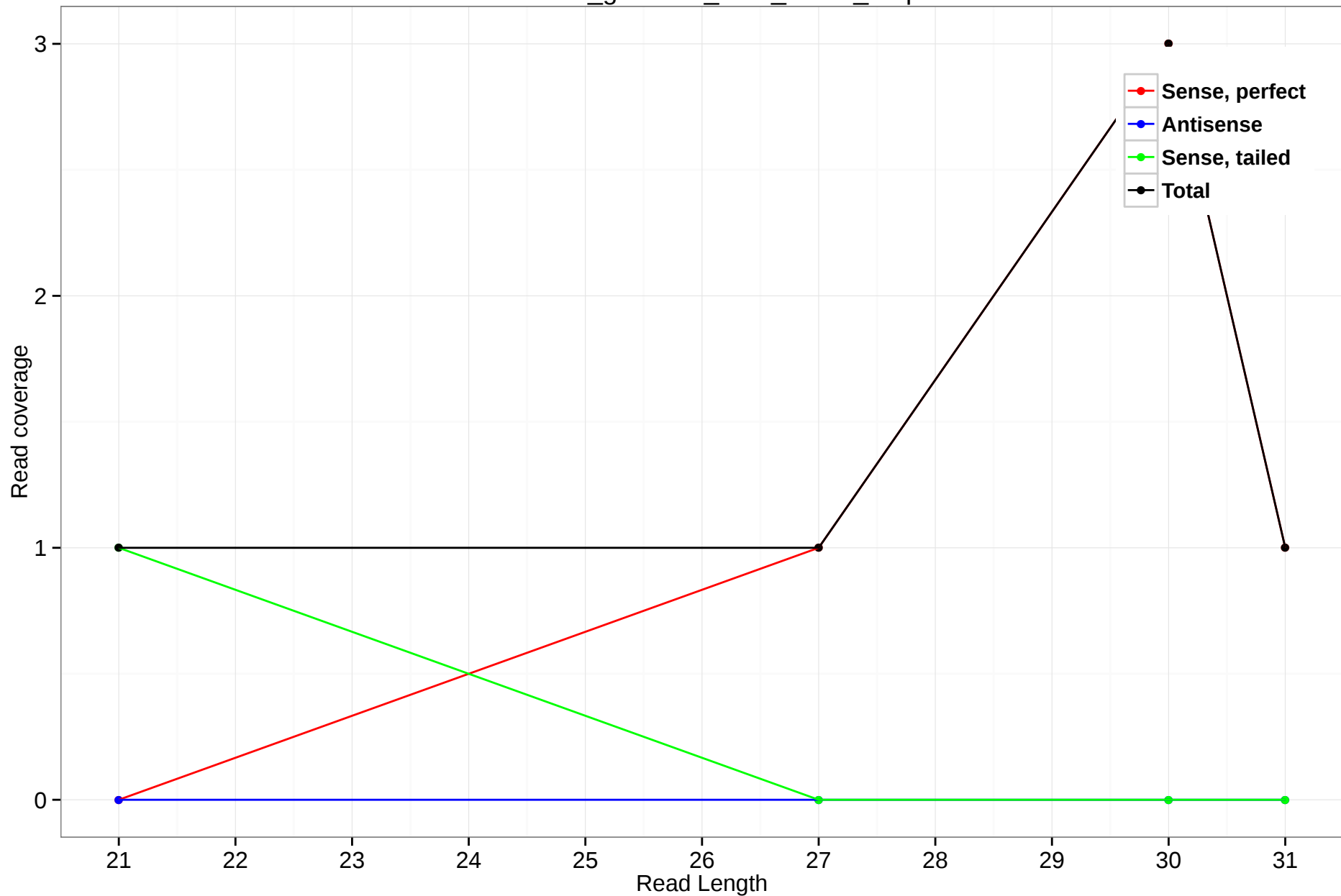
rheMac3_genscan_chr3_248.7_1.5p
