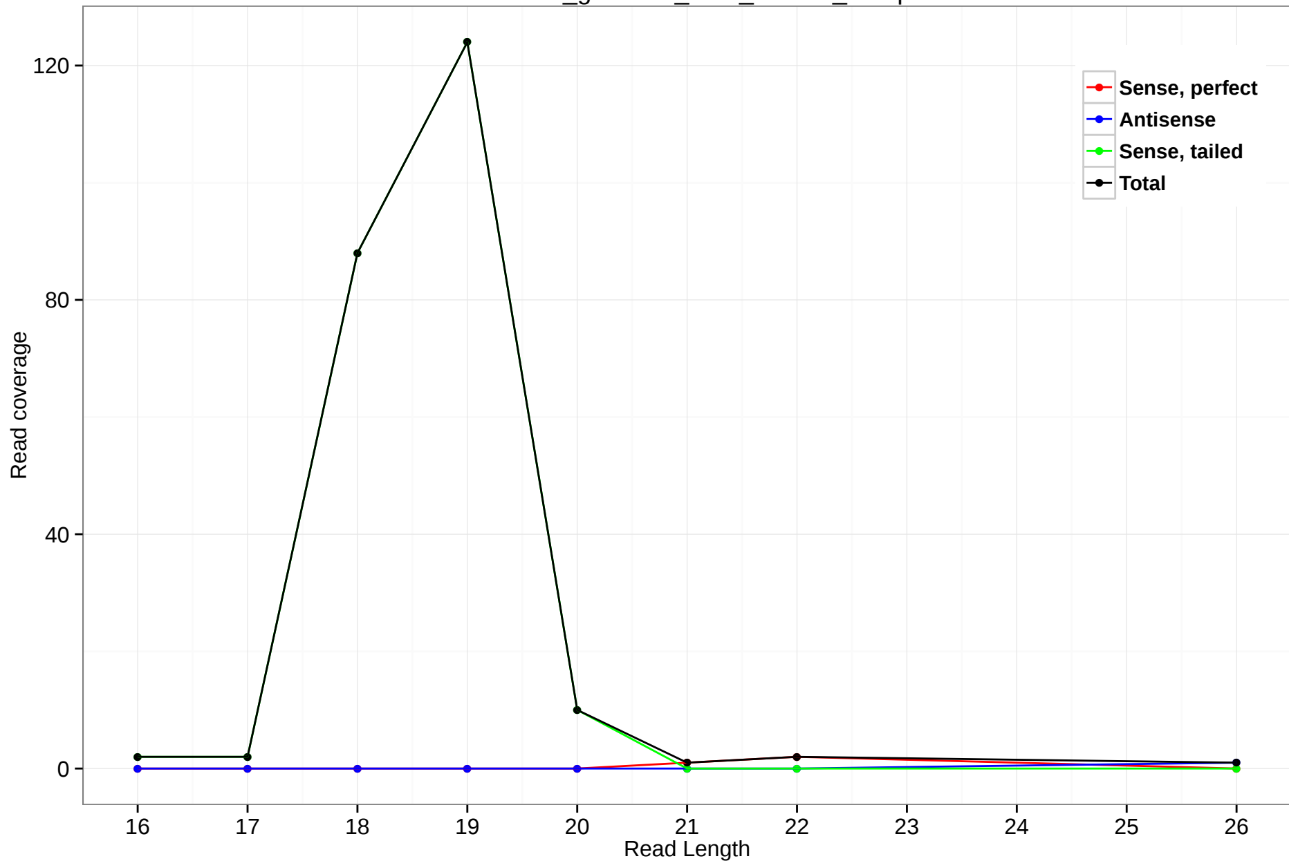
rheMac3_genscan_chr3_247.90_29.3p
