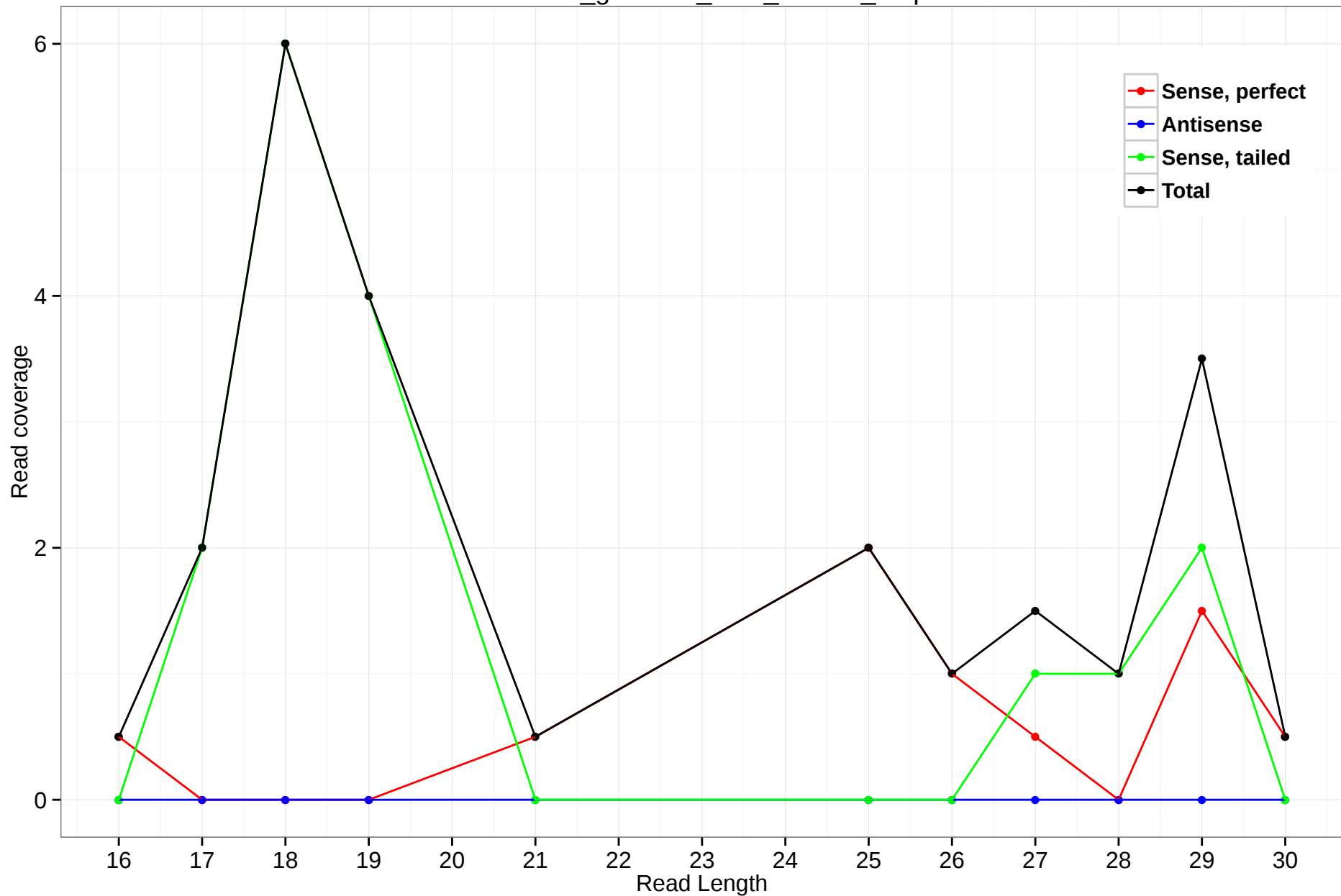
rheMac3_genscan_chr3_247.23_0.5p
