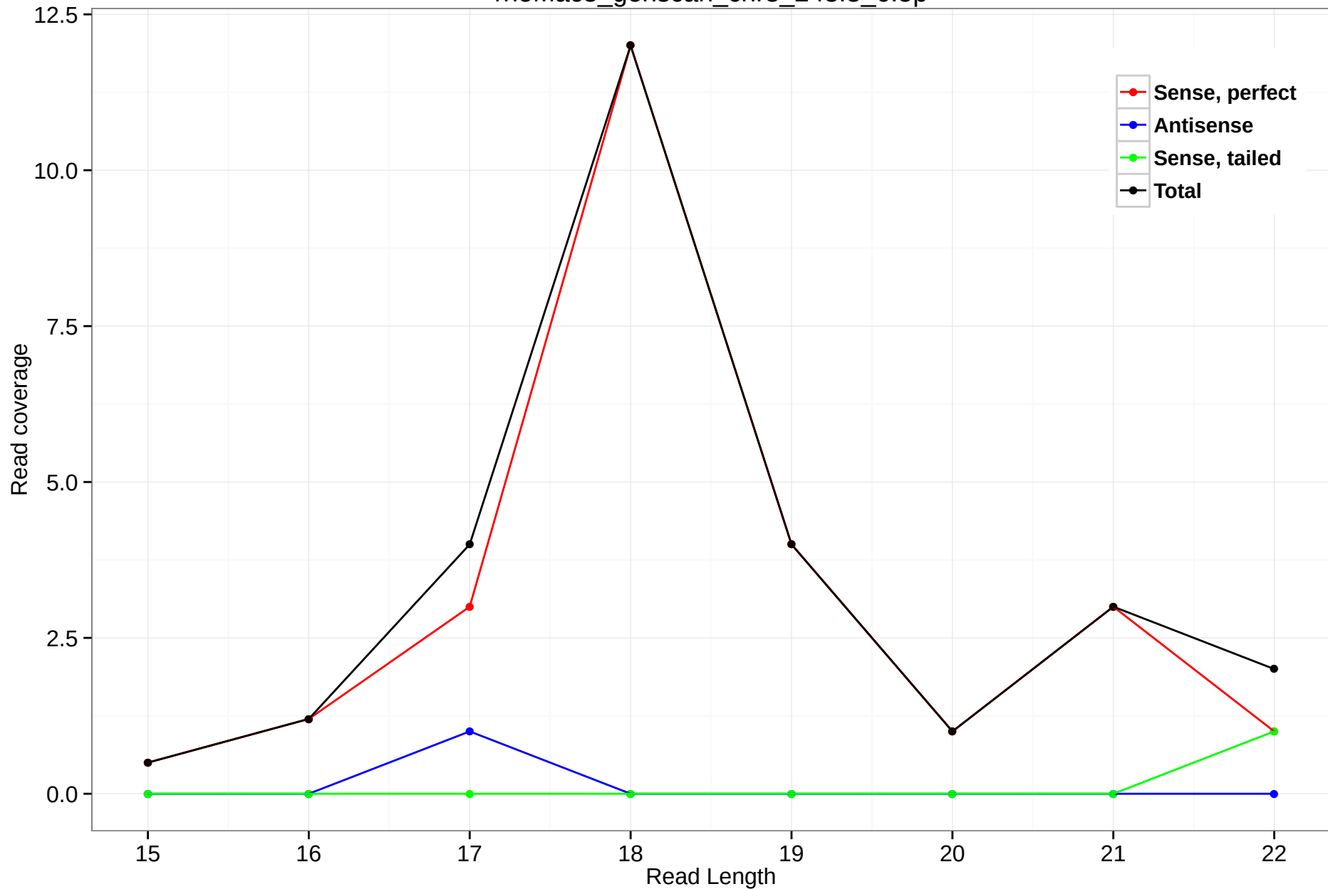
rheMac3_genscan_chr3_243.8_6.5p
