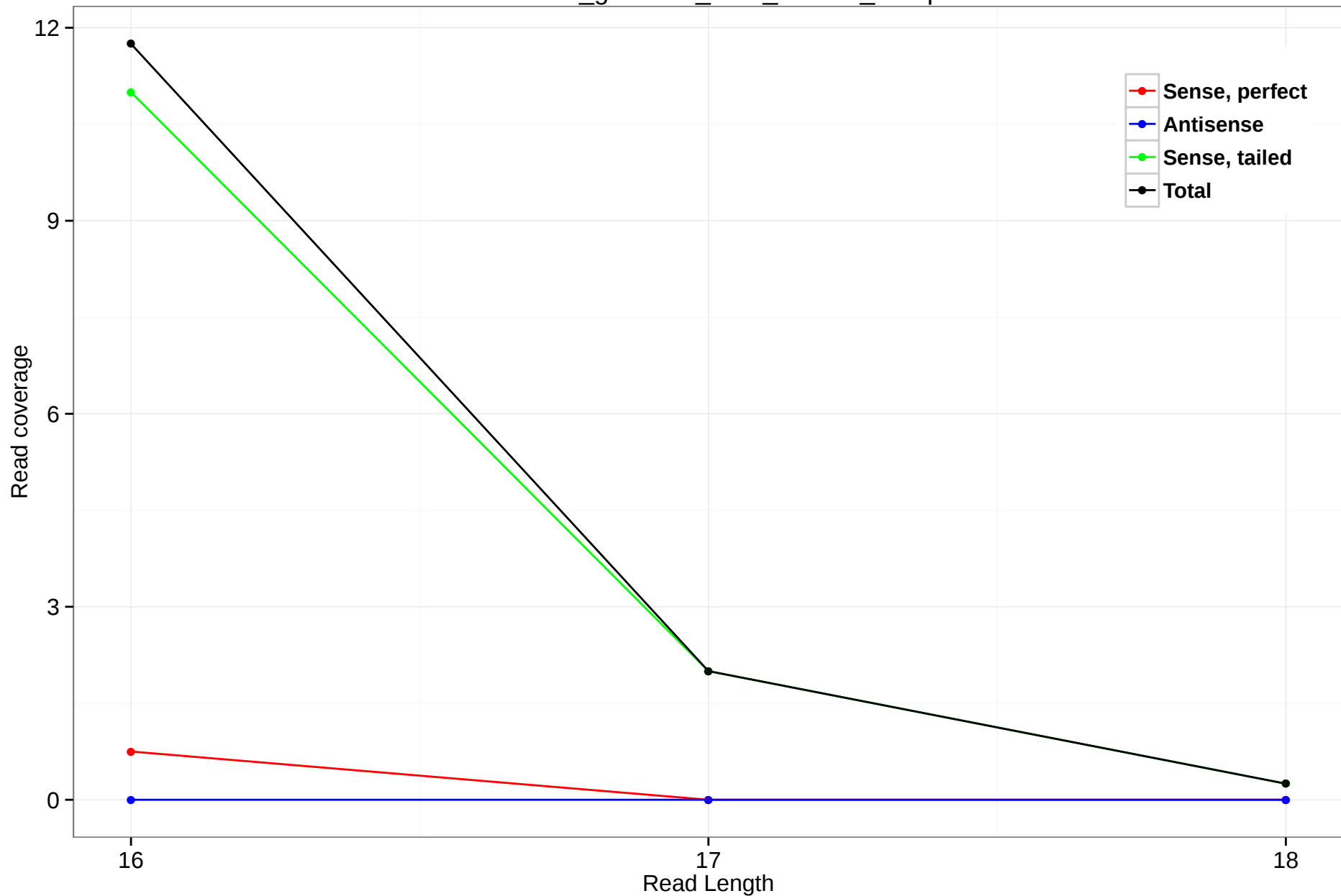
rheMac3_genscan_chr3_238.12_21.5p
