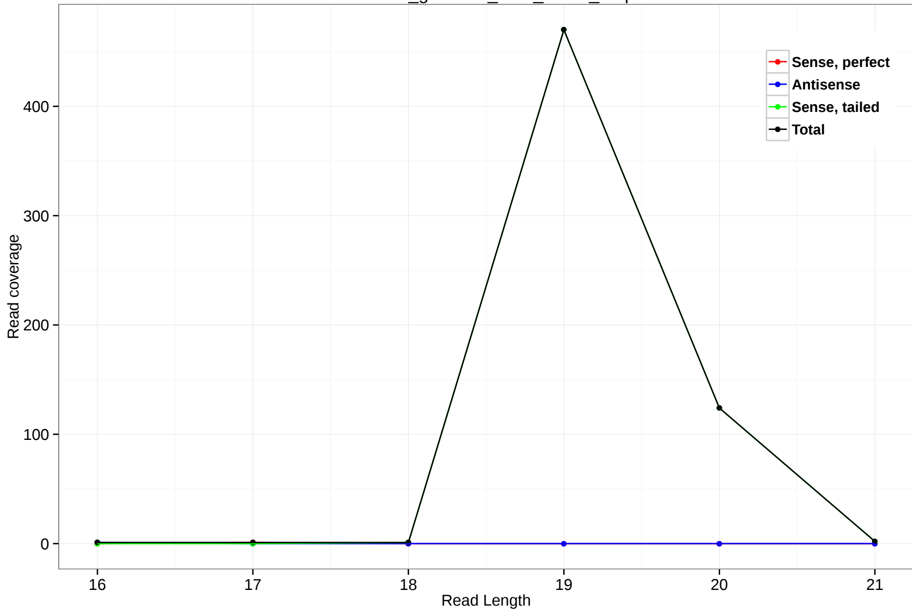
rheMac3_genscan_chr3_218.7_9.3p
