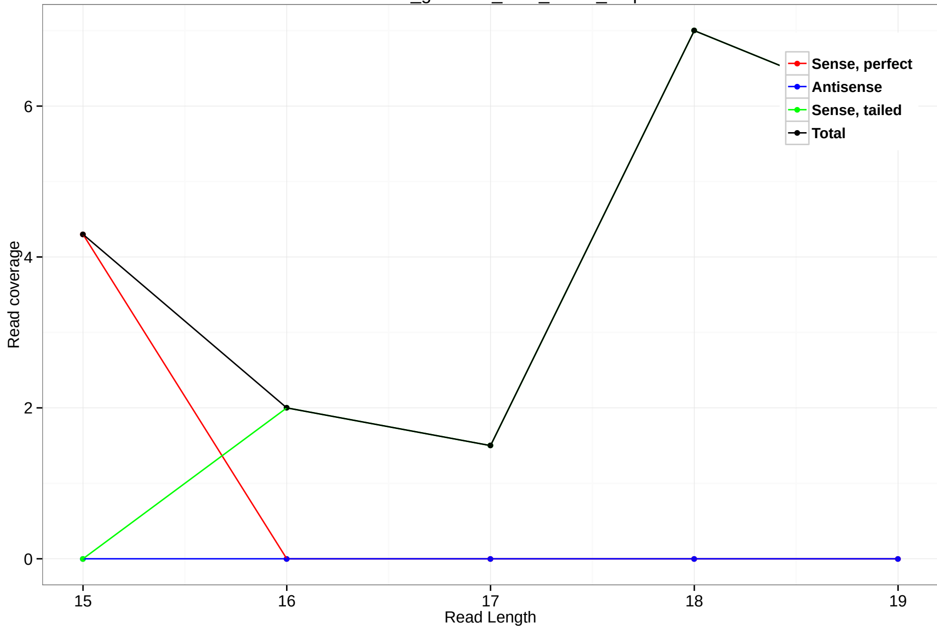
rheMac3_genscan_chr3_212.9_1.5p
