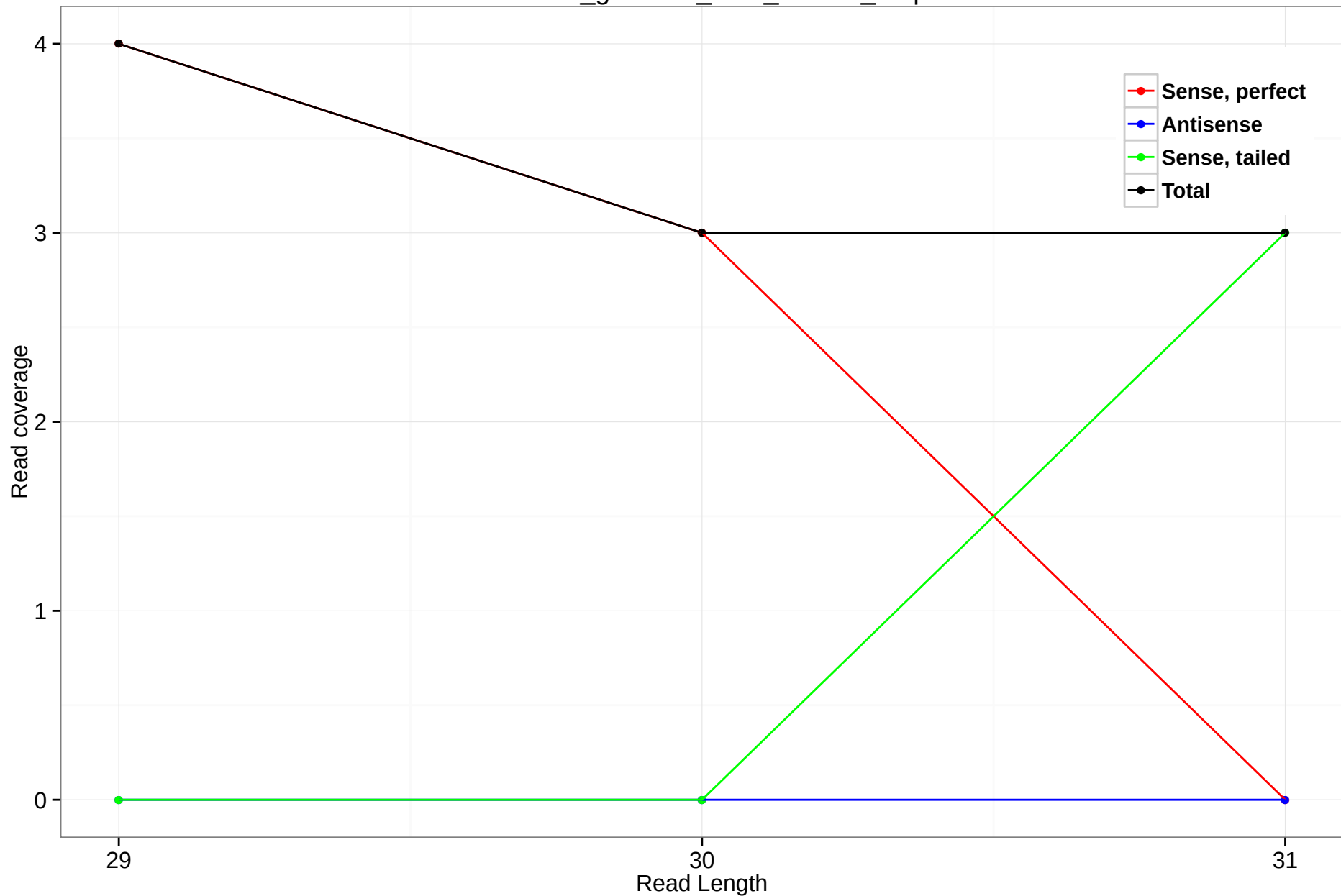
rheMac3_genscan_chr3_212.20_9.3p
