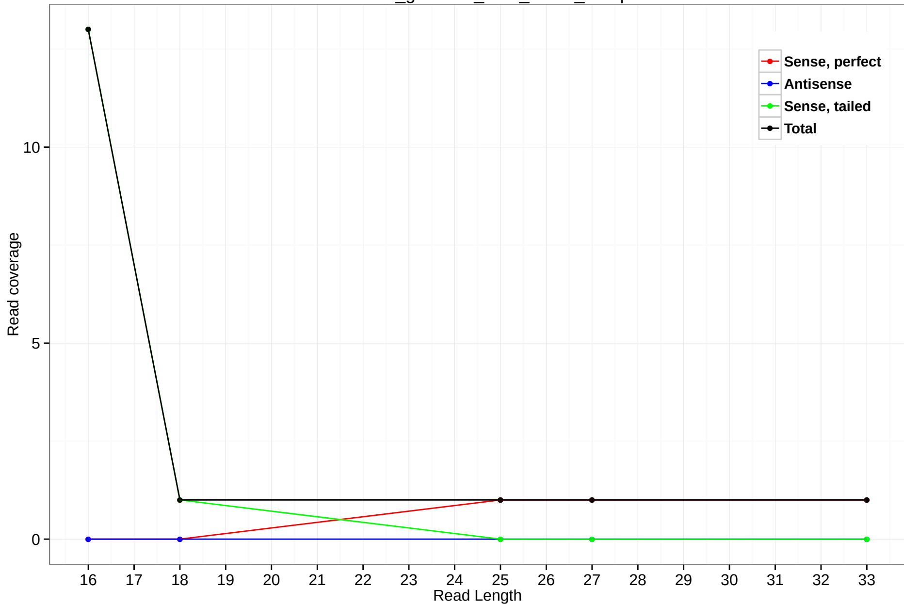
rheMac3_genscan_chr3_21.37_36.5p
