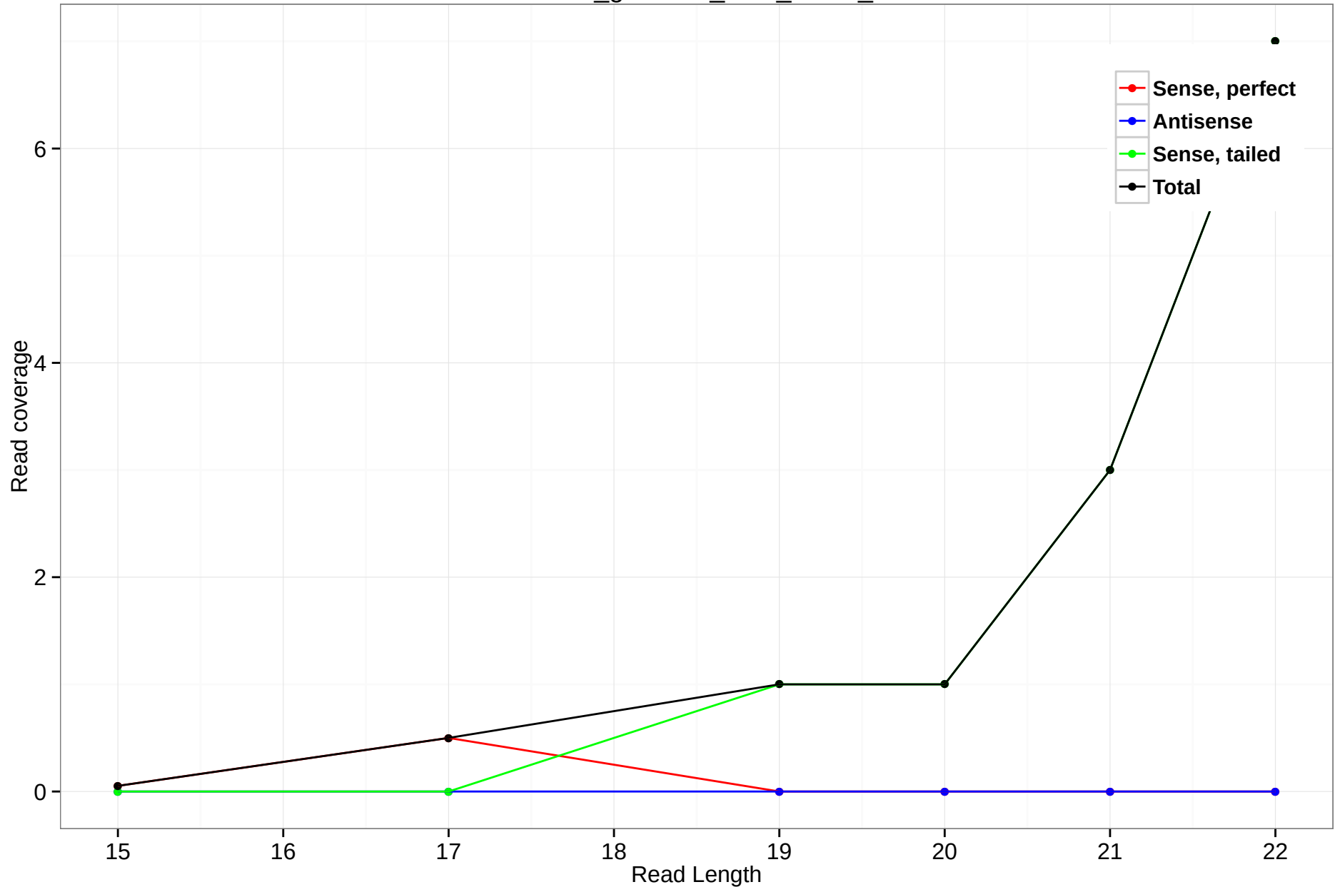
rheMac3_genscan_chr3_21.10_11
