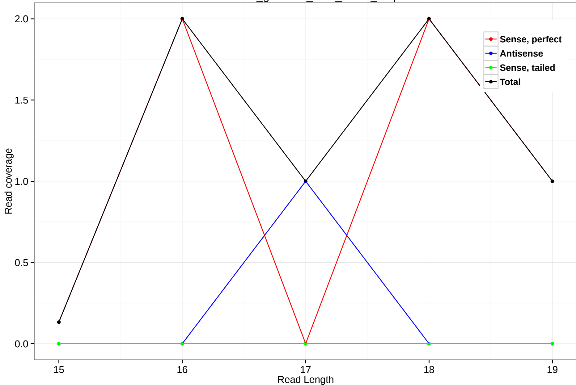
rheMac3_genscan_chr3_197.9_2.5p
