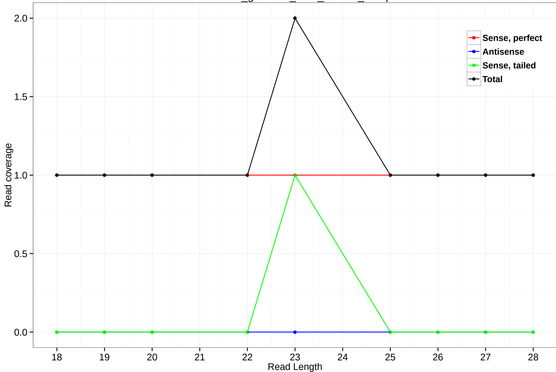
rheMac3_genscan_chr3_197.10_10.3p
