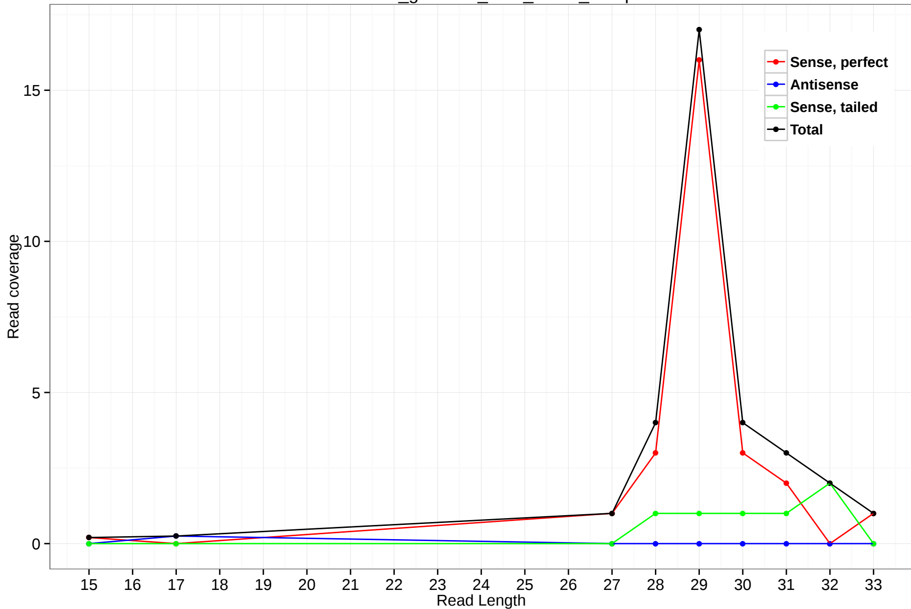
rheMac3_genscan_chr3_196.7_14.3p
