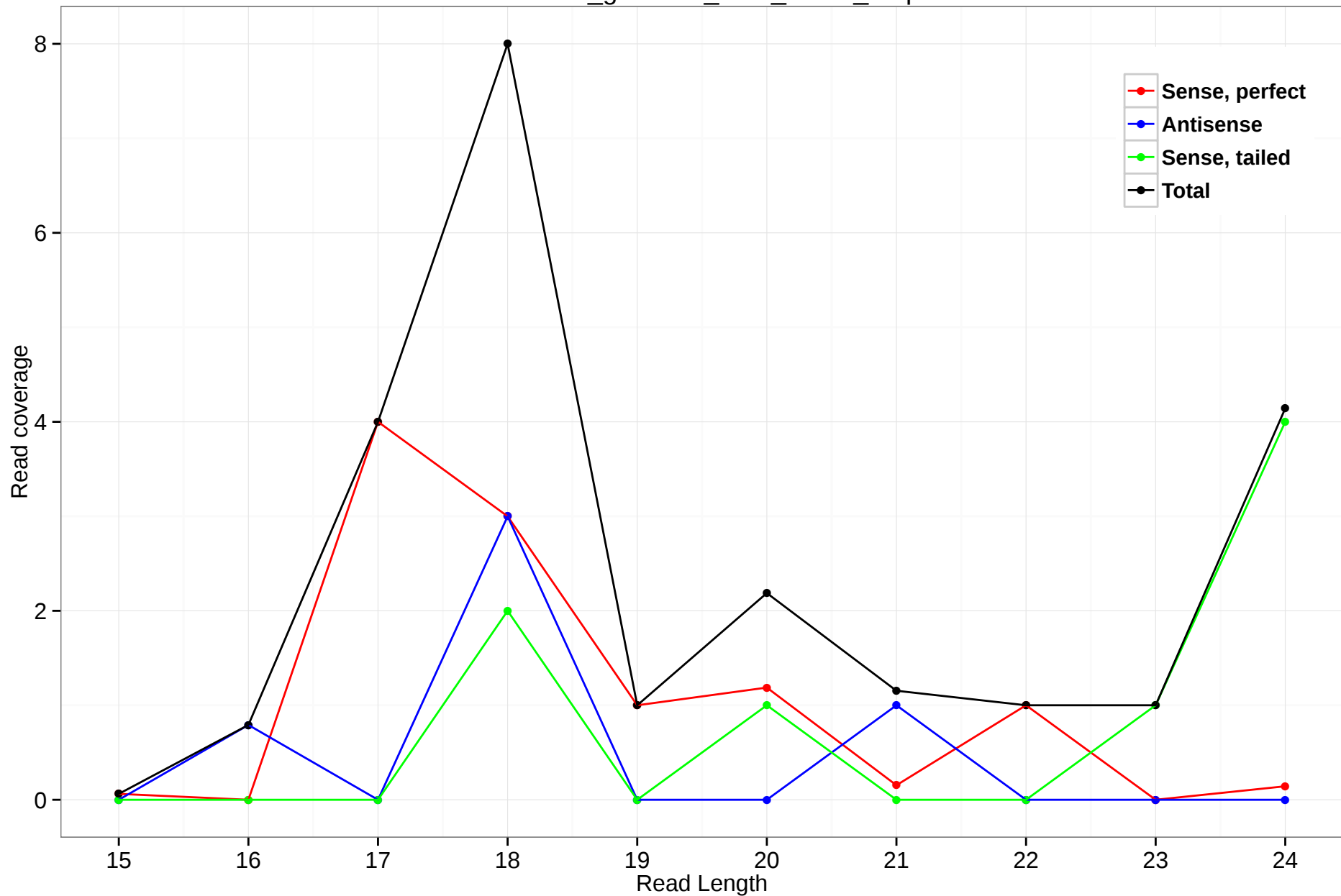
rheMac3_genscan_chr3_160.3_2.5p
