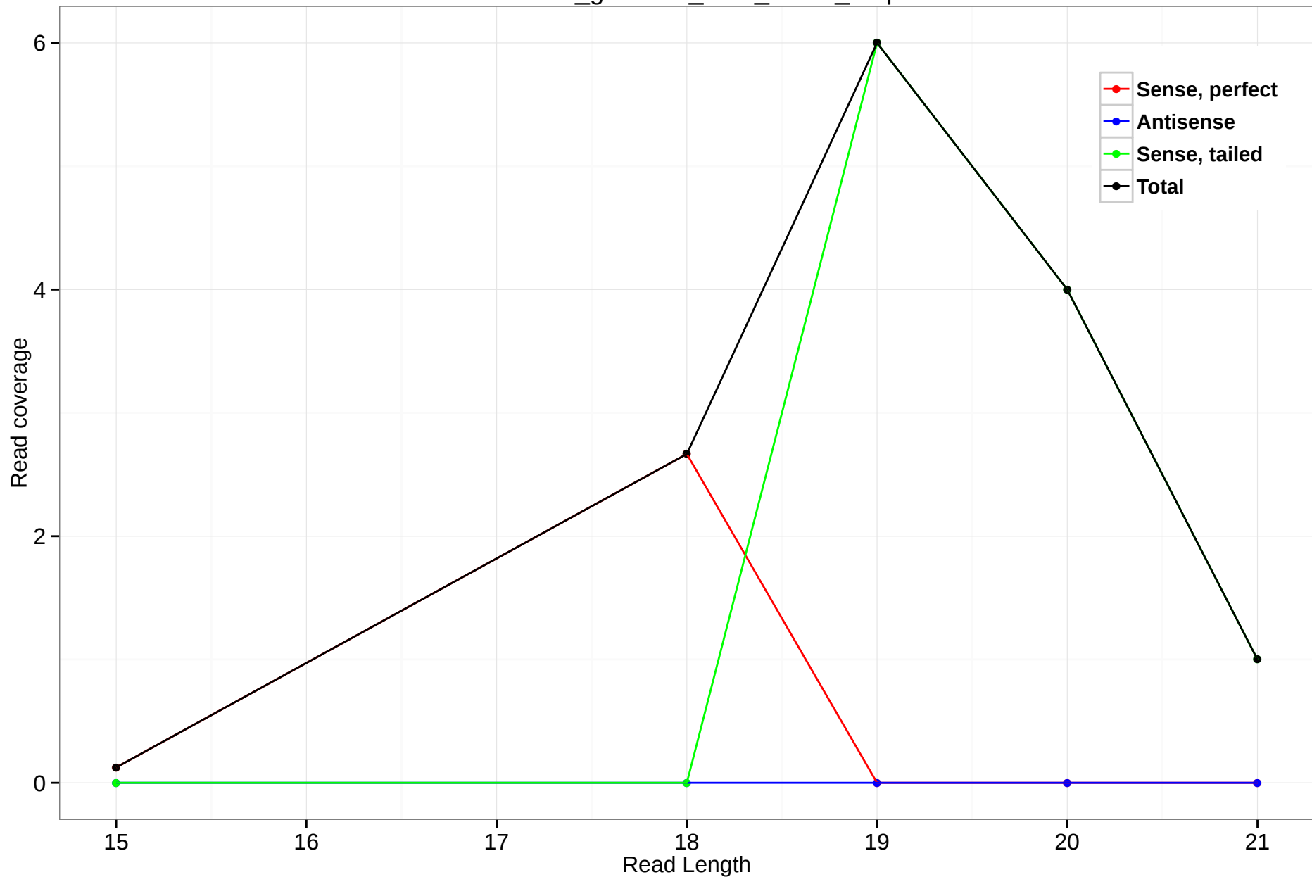
rheMac3_genscan_chr3_16.65_1.3p
