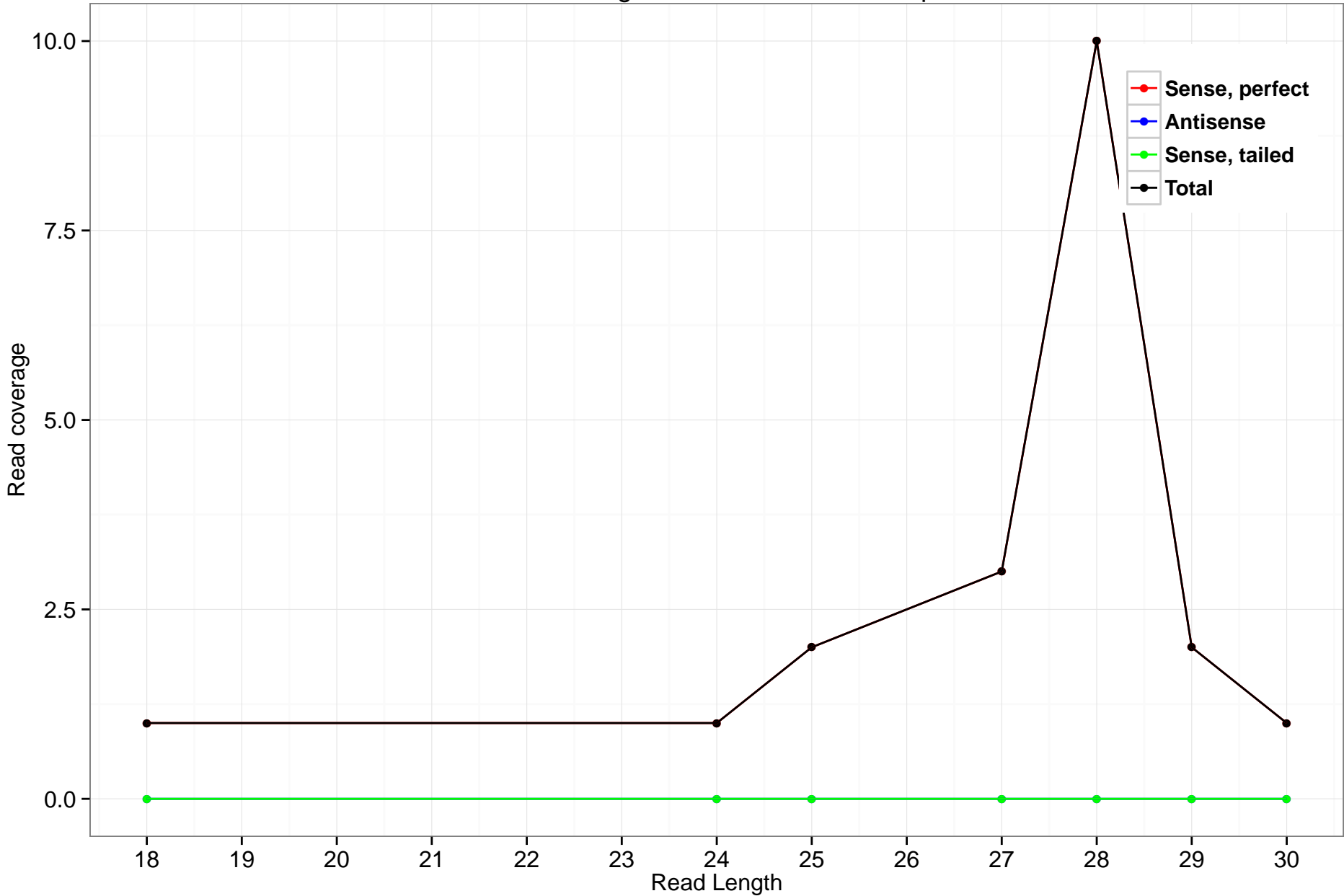
rheMac3_genscan_chr3_16.16_1.5p
