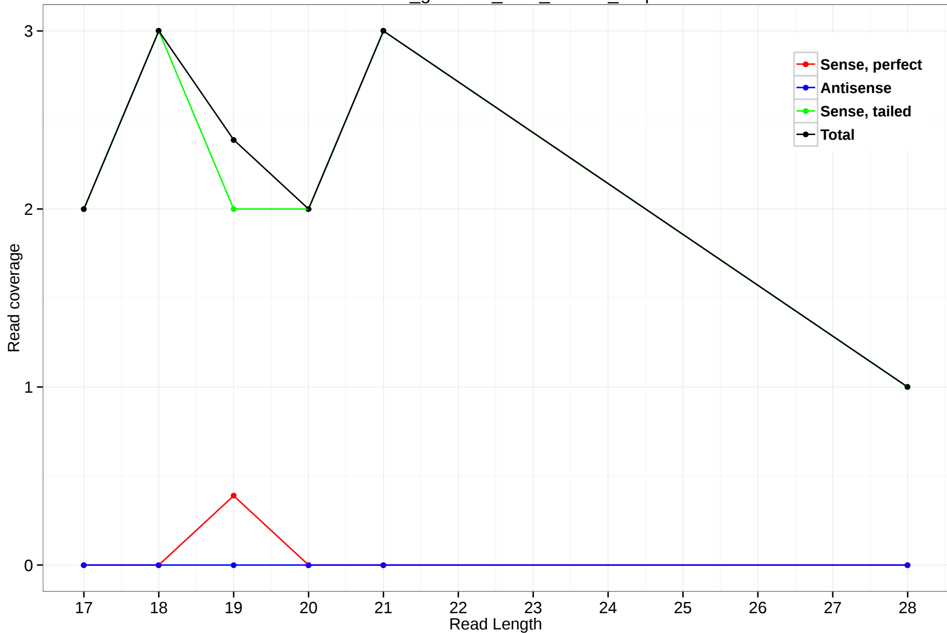
rheMac3_genscan_chr3_159.17_6.5p
