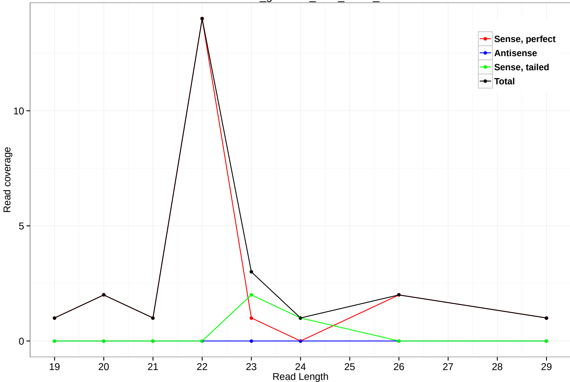
rheMac3_genscan_chr3_155.5_2
