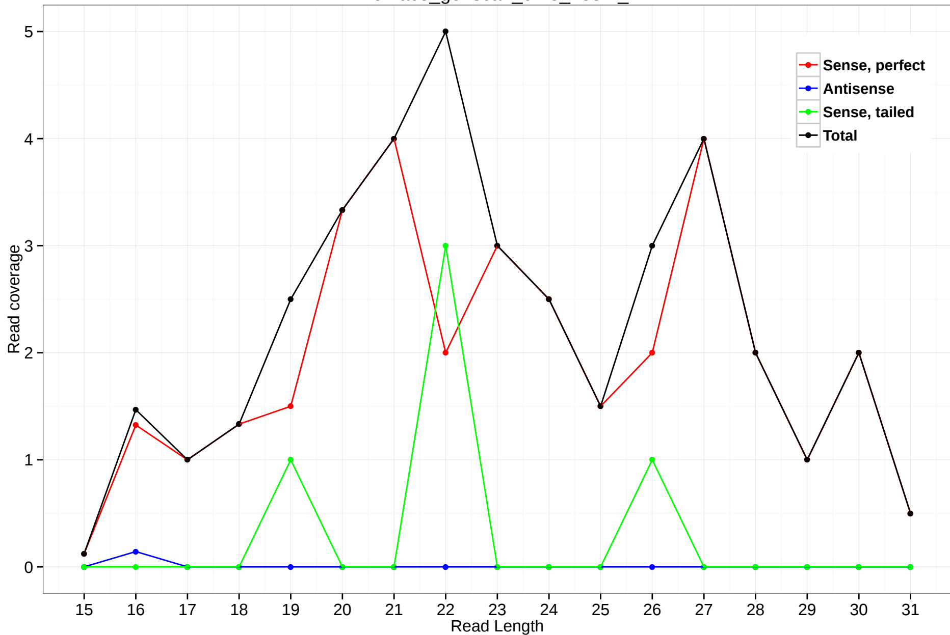
rheMac3_genscan_chr3_155.4_7
