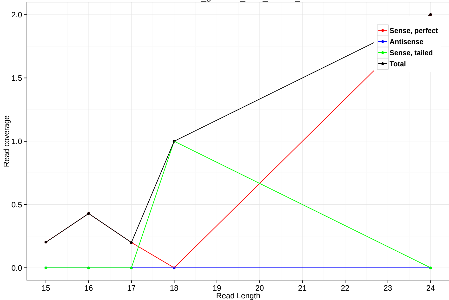
rheMac3_genscan_chr3_155.21_15
