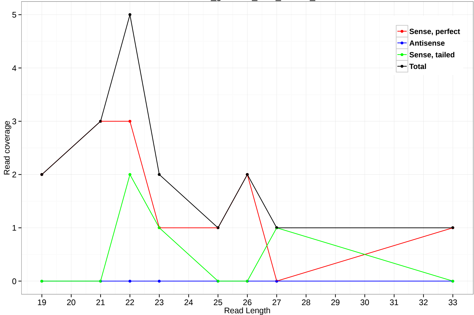
rheMac3_genscan_chr3_155.20_3
