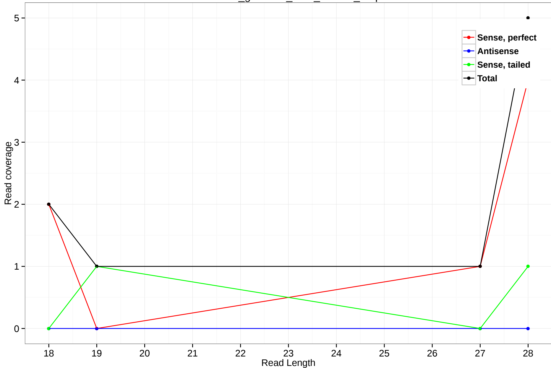
rheMac3_genscan_chr3_155.18_5.3p
