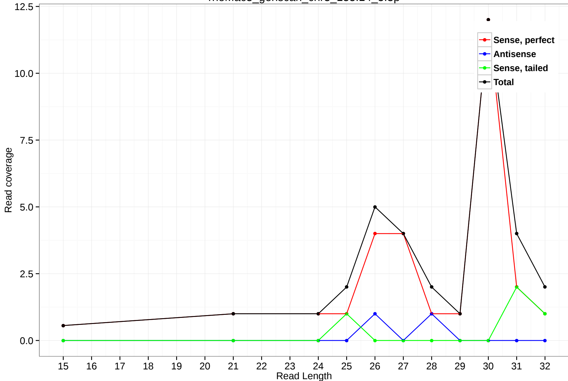
rheMac3_genscan_chr3_155.14_5.3p
