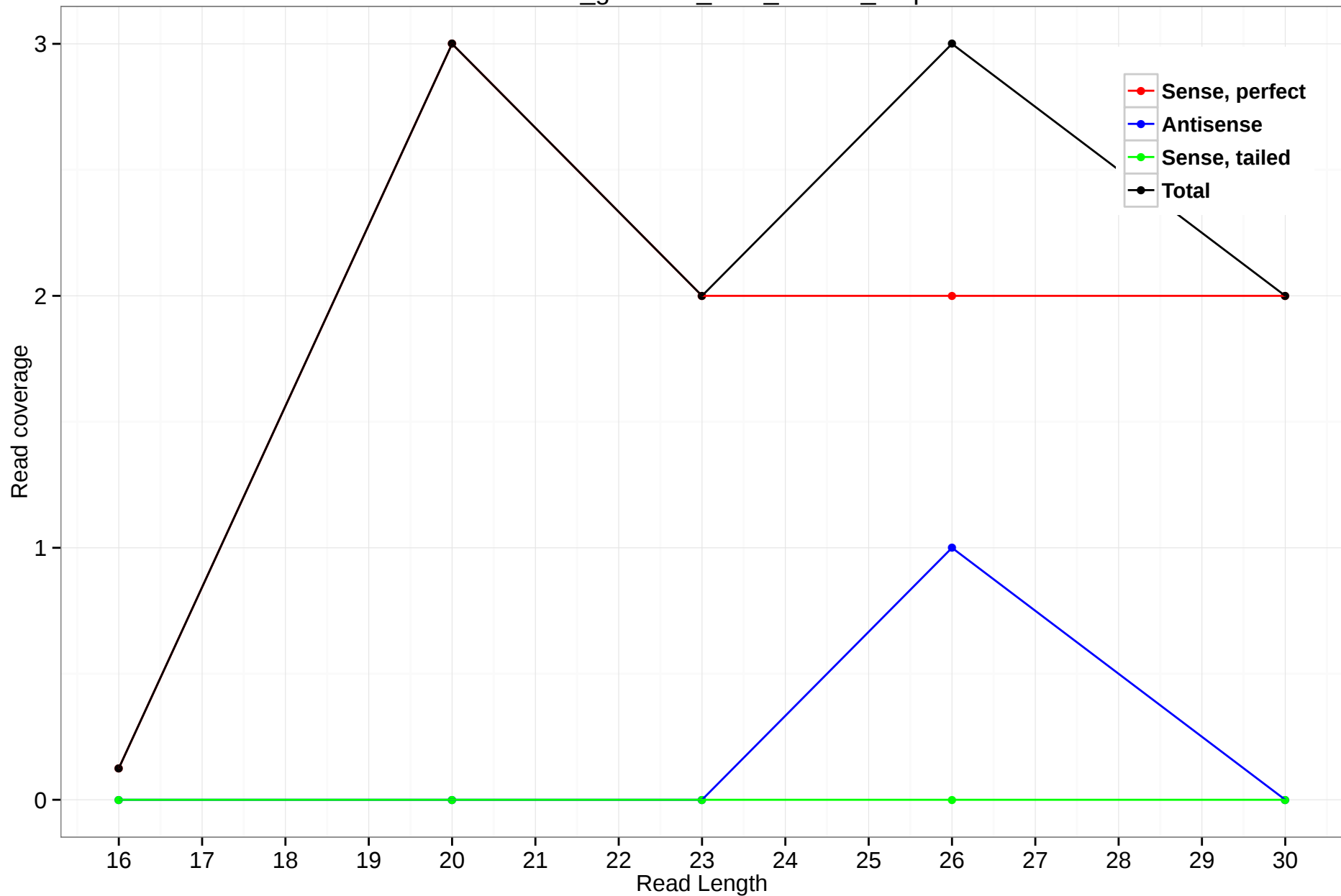
rheMac3_genscan_chr3_155.12_4.5p
