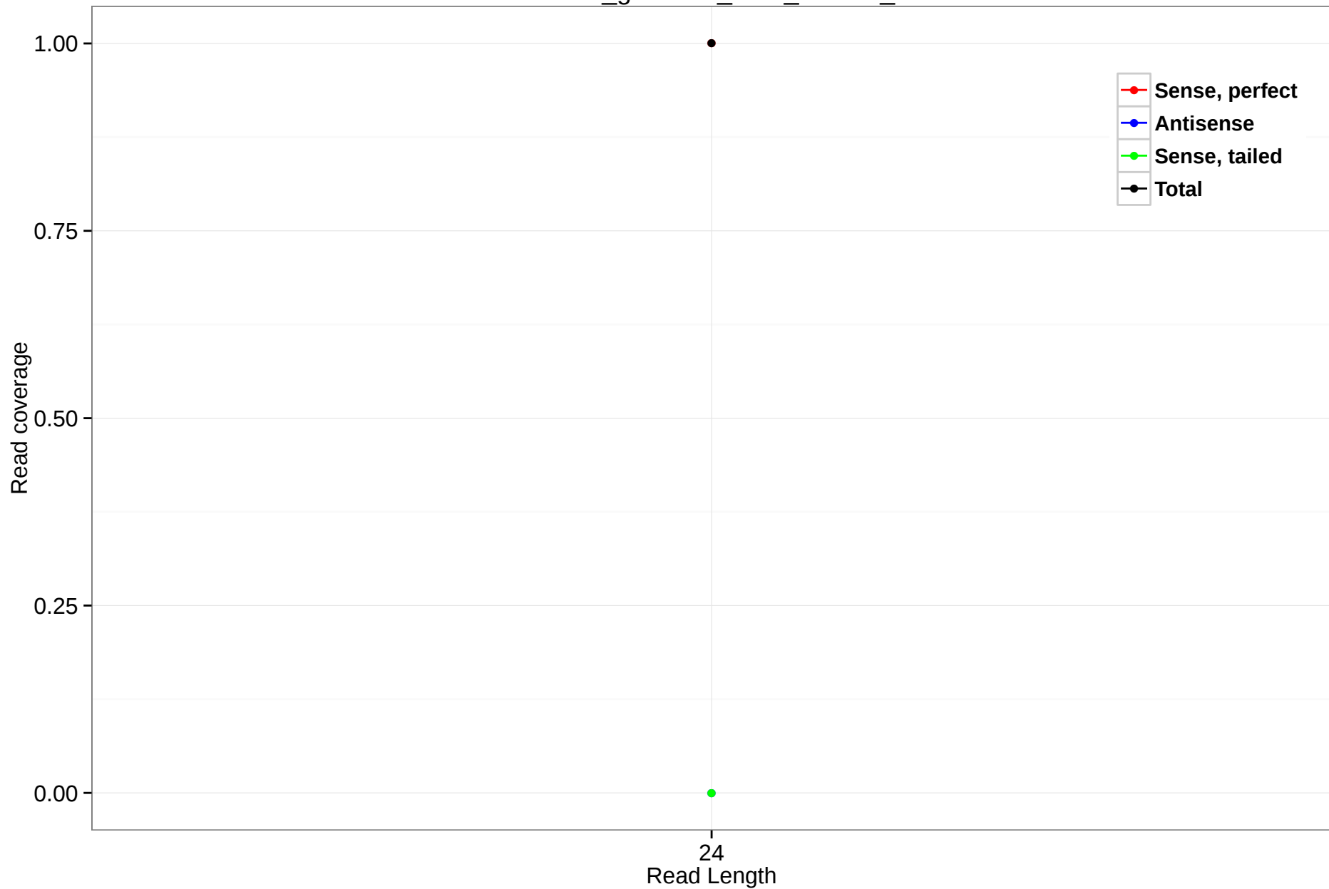
rheMac3_genscan_chr3_155.12_13
