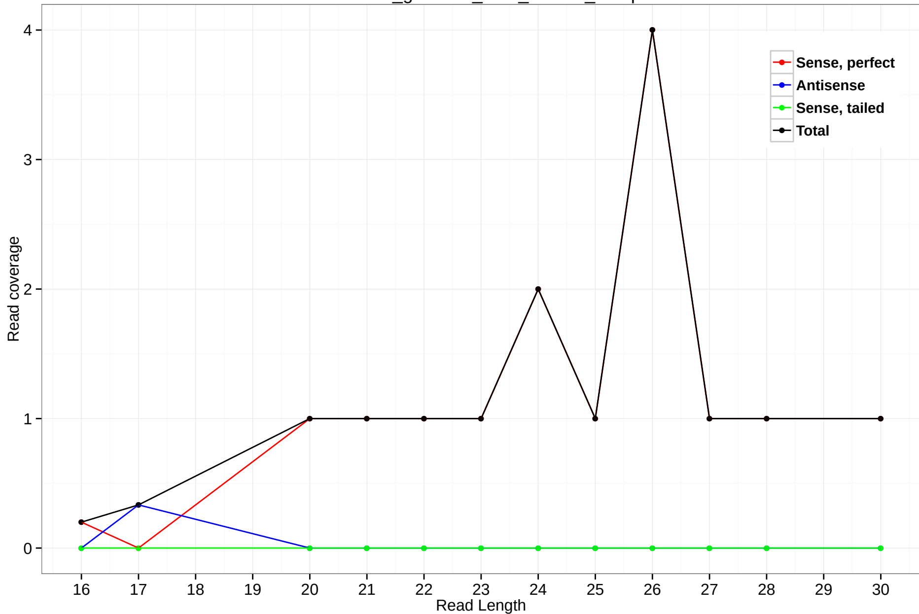
rheMac3_genscan_chr3_154.24_31.5p
