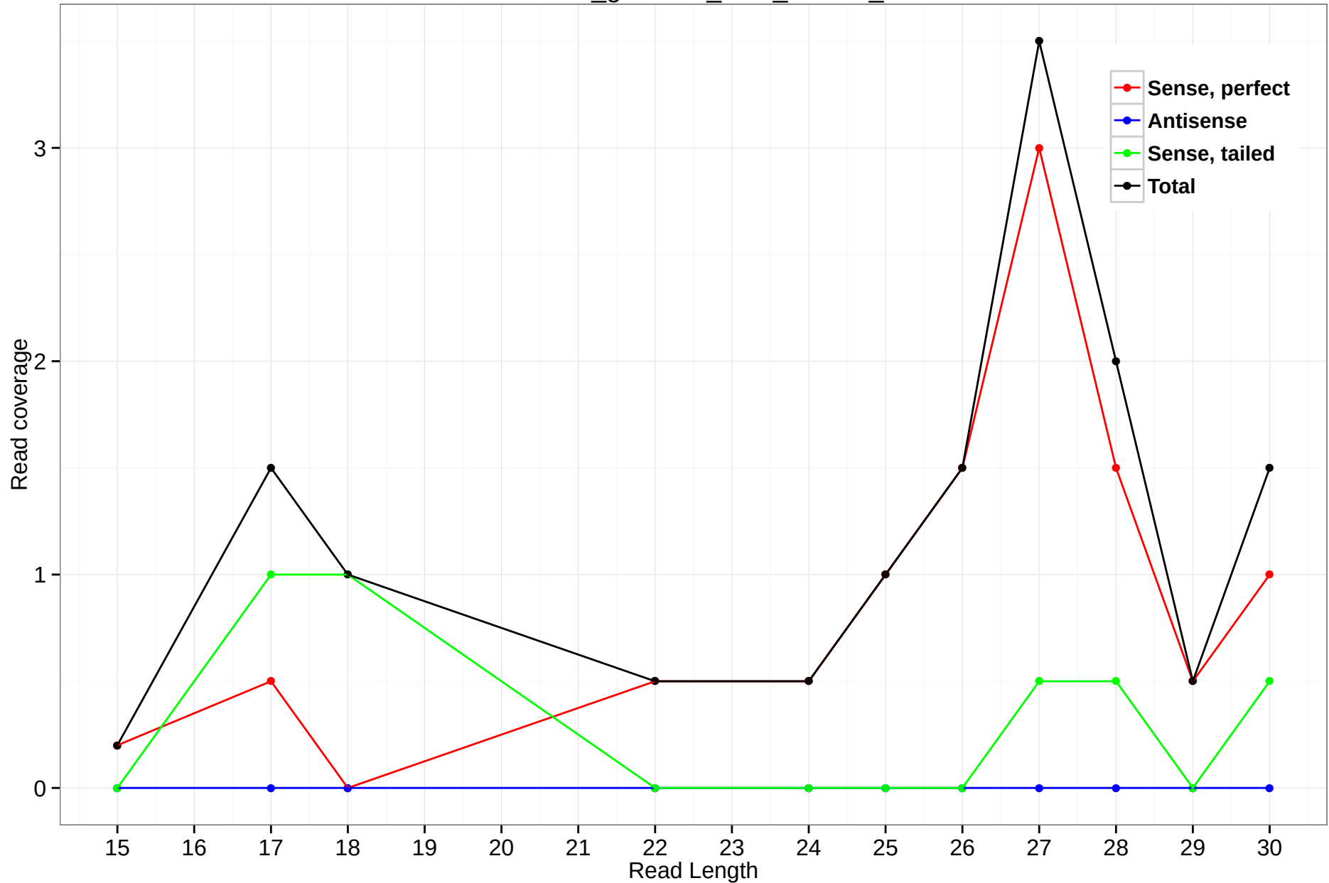
rheMac3_genscan_chr3_150.18_1
