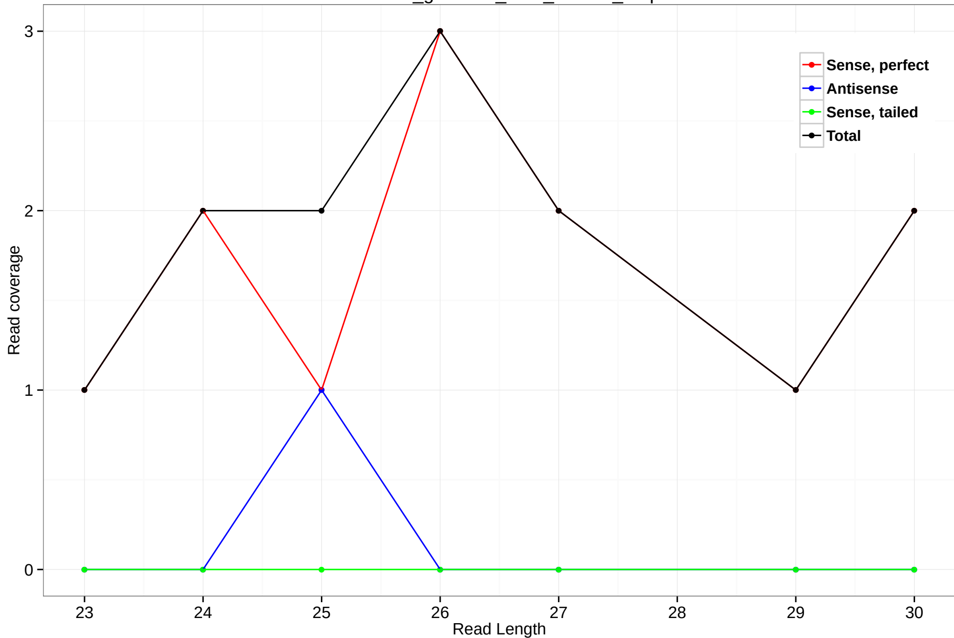
rheMac3_genscan_chr3_146.14_2.5p
