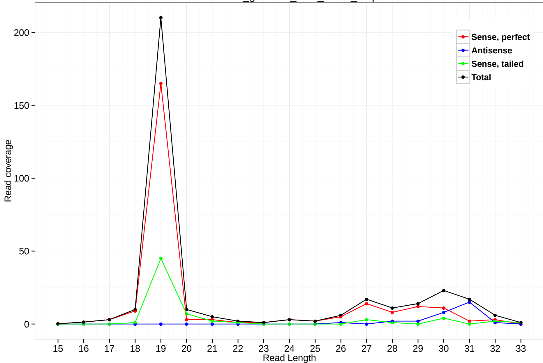
rheMac3_genscan_chr3_112.1_1.3p
