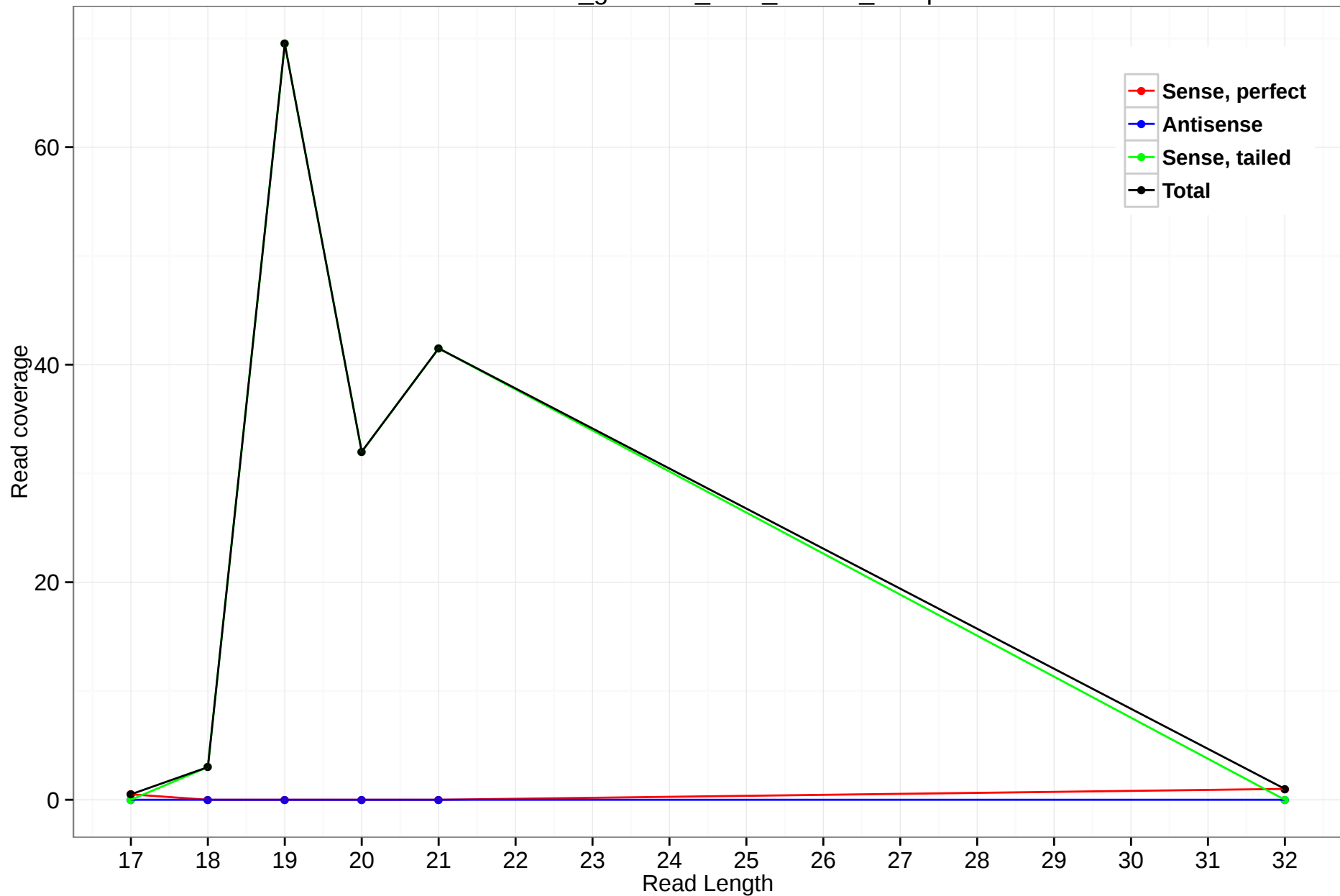
rheMac3_genscan_chr3_106.47_12.3p
