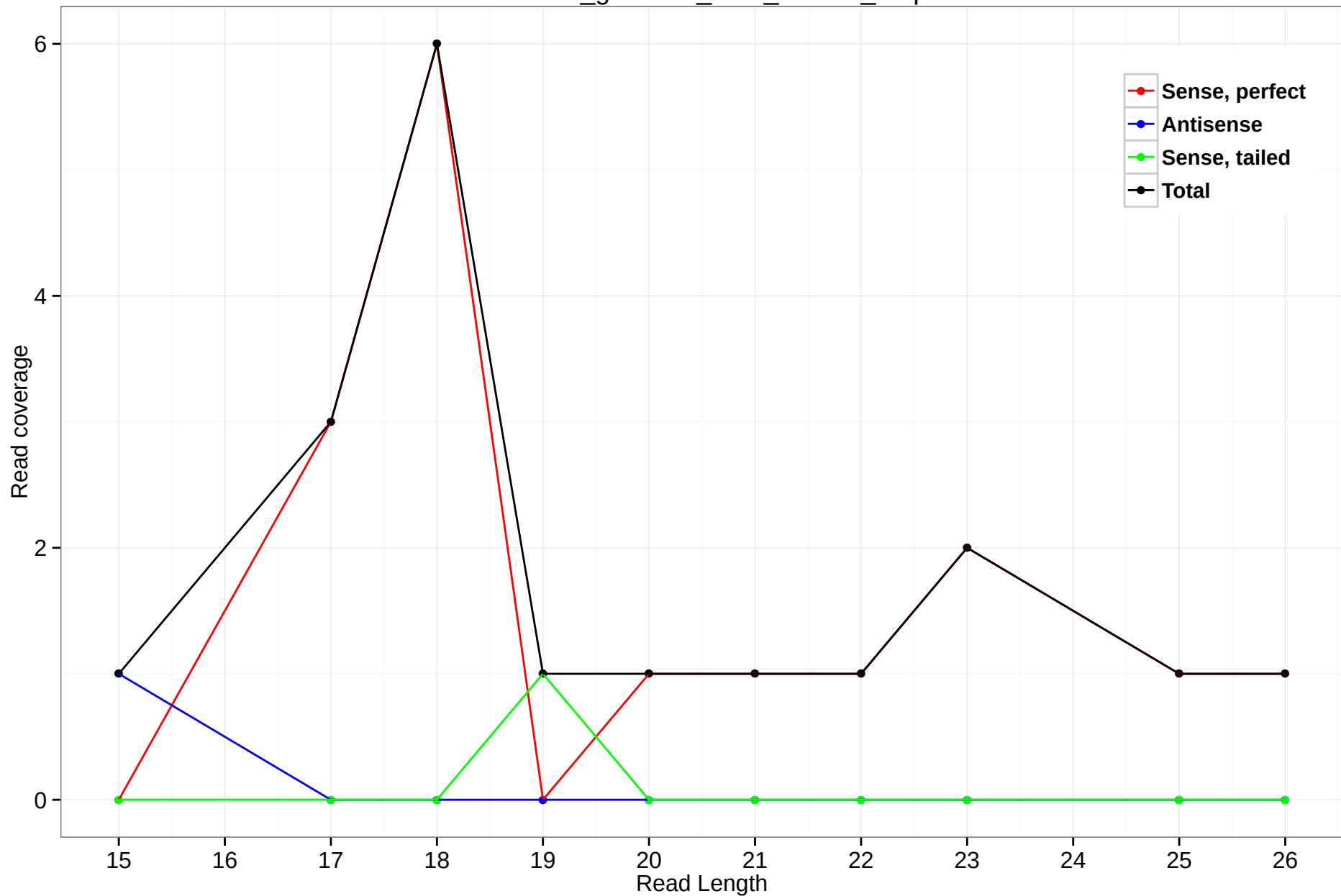
rheMac3_genscan_chr3_106.38_2.5p
