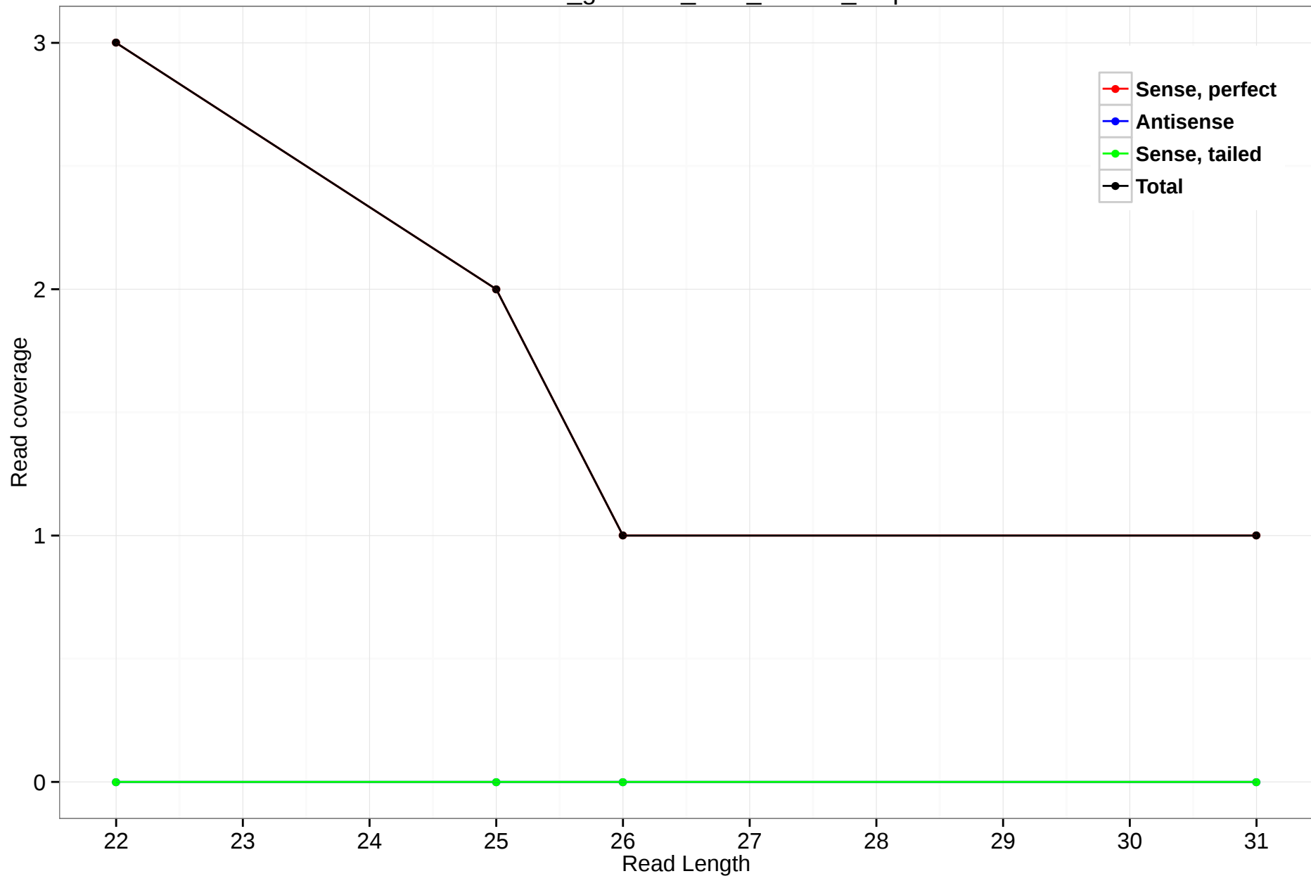
rheMac3_genscan_chr3_106.10_6.3p
