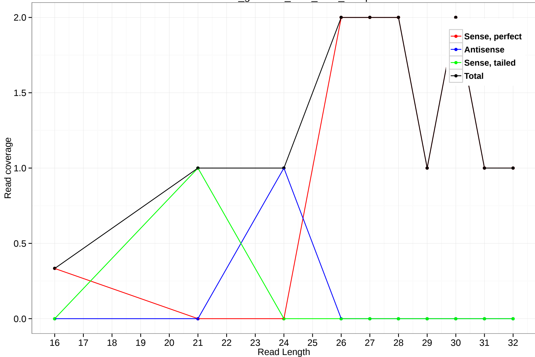
rheMac3_genscan_chr3_08.7_25.5p
