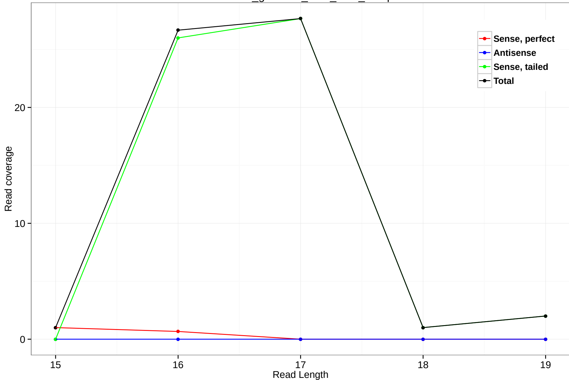
rheMac3_genscan_chr3_05.6_15.5p
