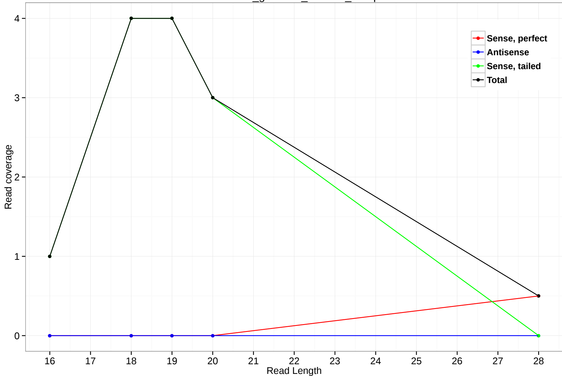
rheMac3_genscan_chr3.19_24.3p
