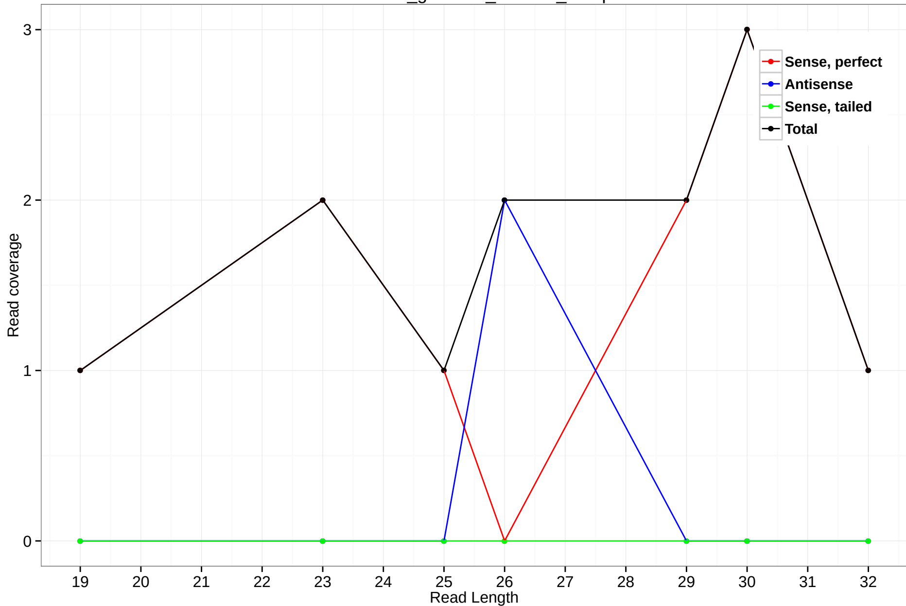
rheMac3_genscan_chr3.19_23.5p
