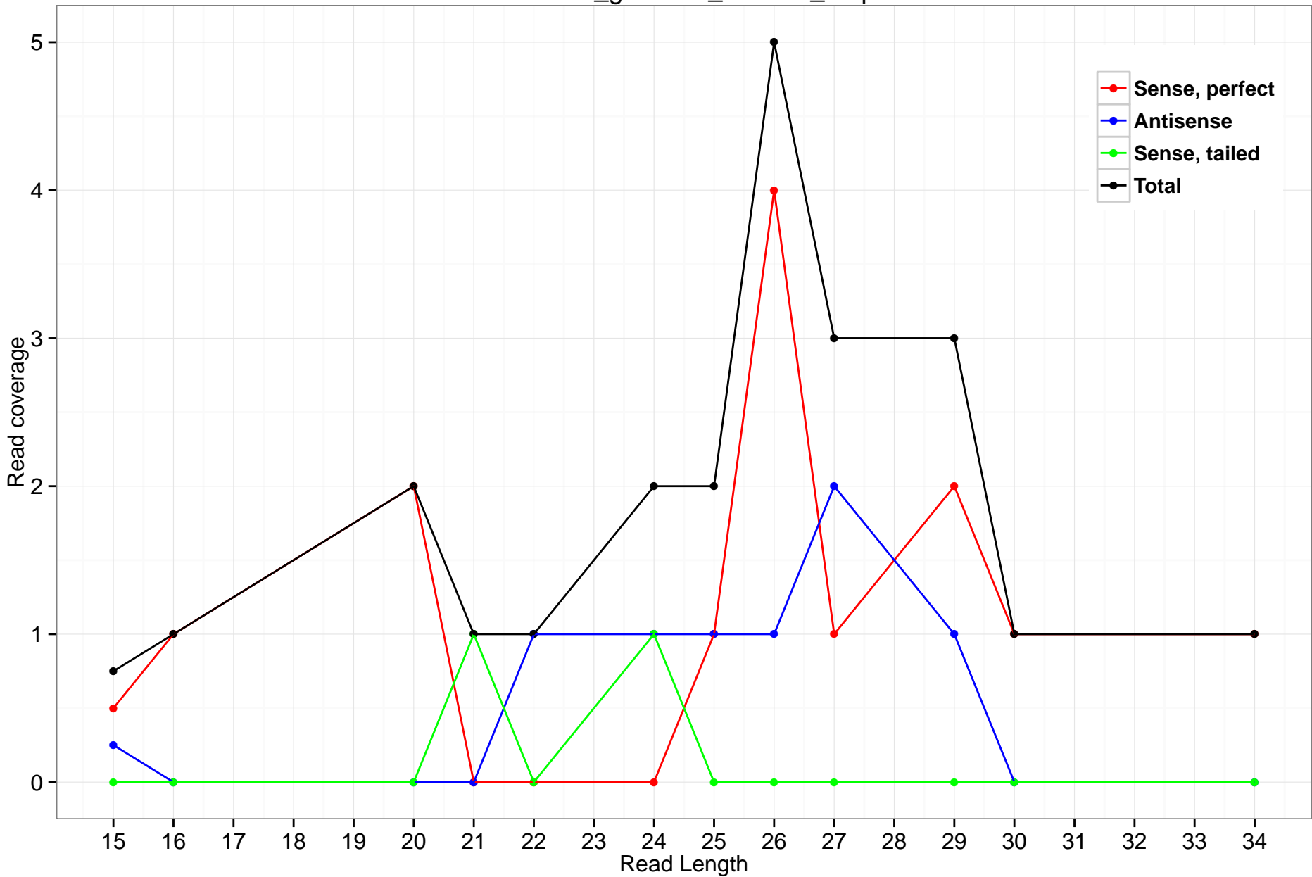
rheMac3_genscan_chr3.18_4.5p
